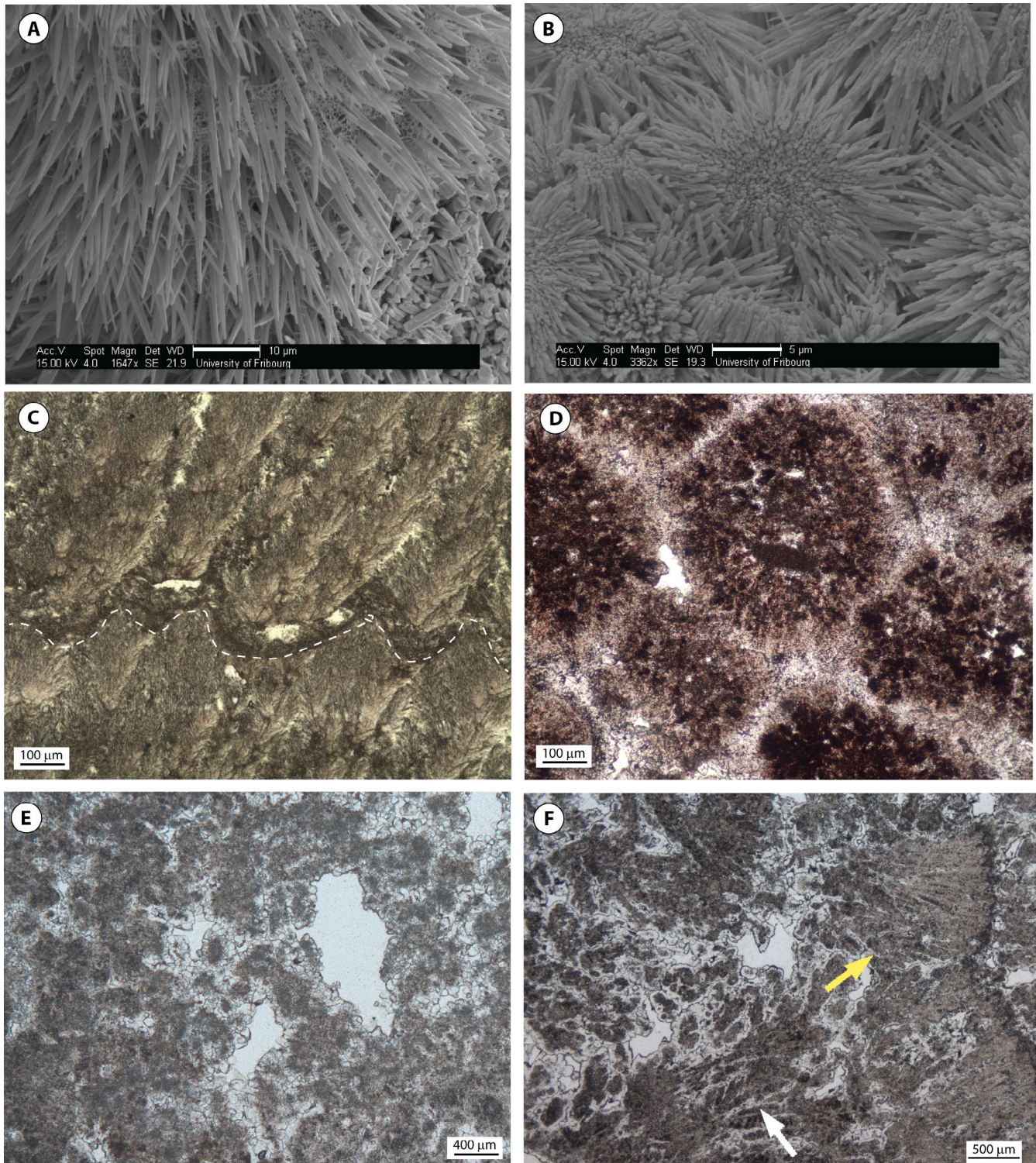
FIGURE 3 Petrography of modern and fossil travertine deposits. (A) Aragonite needles radiating out from a fossilized microbial filament in the Apron-Channel facies at New Grassy spring. Between the needles, fossilized EPS can be seen that connects the needles and forms a honeycomb network (SEM-SE). (B) Fine aragonite needles forming spherules in a Distal Slope sample at Narrow Gauge spring (SEM-SE). (C) Transmitted light image of aragonite shrub textures in a Proximal Slope sample from the Narrow Gauge spring. The dotted line outlines a microterraccete front with some silt-sized grains deposited along it. (D) Transmitted light image of spherules in a Distal Slope facies section of the Y-10 core (sample 27). (E) Transmitted light image of micritic to peloidal fabric, surrounded by a transparent calcite cement rim that occurs together with the spherules of image D (Y-10, sample 27). (F) Different dendritic textures co-occurring in a Proximal Slope sample. Poorly branching dendritic textures on the left (white arrow) give way to more crystal ray fans to the right (yellow arrow; Y-10, sample 37)
