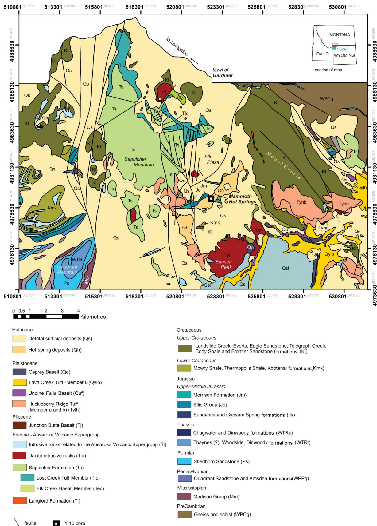
FIGURE 1 Geological map of the northern part of Yellowstone National Park with the location of Mammoth Hot Springs and the Y-10 core (WY, USA). Modified after Christiansen (1999)
