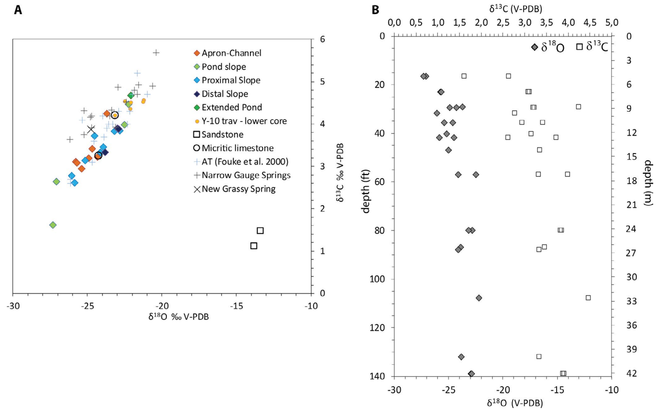
FIGURE 10 Bulk stable carbon and oxygen isotope results. (A) \delta^{13}\text{C} – \delta^{18}\text{O}_{\text{VPDB}} cross-plot of data from the Narrow Gauge springs and the Y-10 core together with data of the MHS system as reported by Fouke et al. (2000). AT, Angel Terrace. (B) \delta^{13}\text{C} and \delta^{18}\text{O}_{\text{VPDB}} data of all travertine samples with depth in the top 42.6 m (140 ft) of the core
