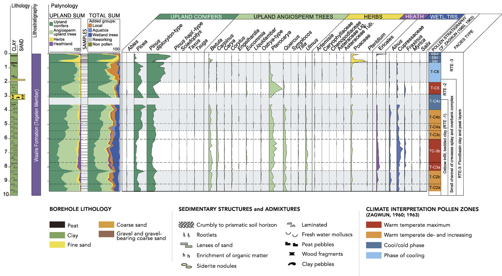
Fig. 11. Lithology, lithostratigraphy, pollen diagram and facies units from the Russel-Tiglia-Egypte pit. Recalculated pollen sums based on data published by Zagwijn (1963a) . Local pollen assemblage zones (PAZ) are delineated by black lines, subzones by black and grey dashed lines. T-zones indicate the classical interpretation based on the definitions of Zagwijn (1960, 1963a) . Alternate grey highlighted zones for visibility. The stratigraphical and climatic interpretations of the pollen zones are derived from the original publication ( Zagwijn, 1963a ).
