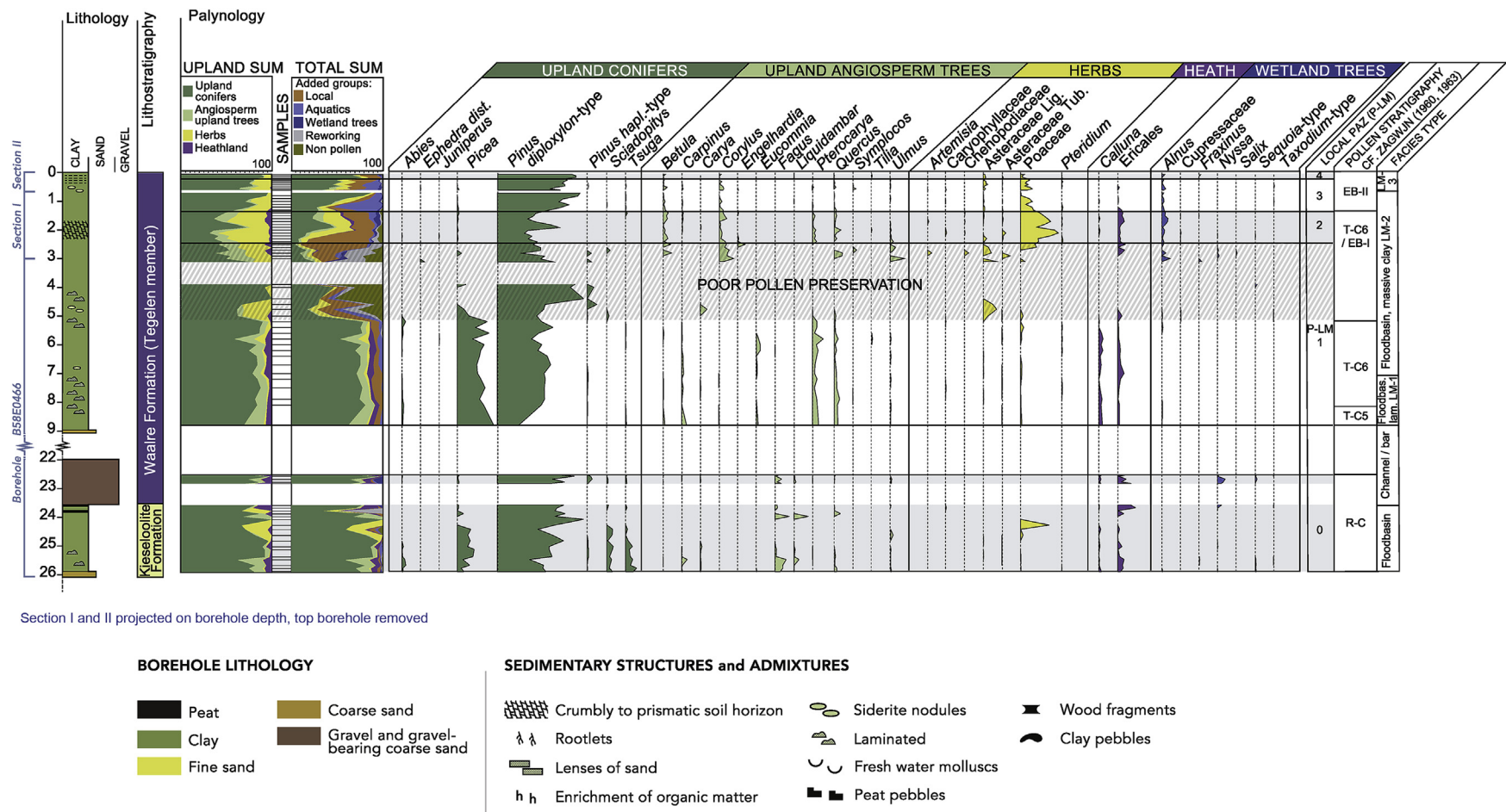
Fig. 10. Lithology, lithostratigraphy, pollen diagram and facies units from the Laumans pit. The upper 3 m of the pollen diagrams are sampled from the sections at the top of the exposed clay deposits (Fig. 9). The lower pollen diagram is derived from borehole B58E0466 that was executed in the pit (see Fig. 9). Local pollen assemblage zones (PAZ) are delineated by black lines, subzones by dashed lines. T-zones indicate the classical interpretation based on the definitions of Zagwijn (1960, 1963a). Alternate grey highlighted zones for visibility.
