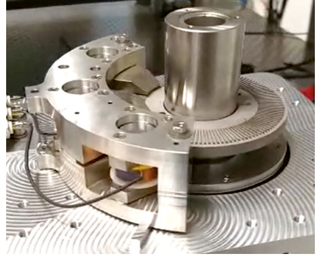
Fig. 7. Photo of the CPA breadboard setup to validate the performance of a single motorization axis.
