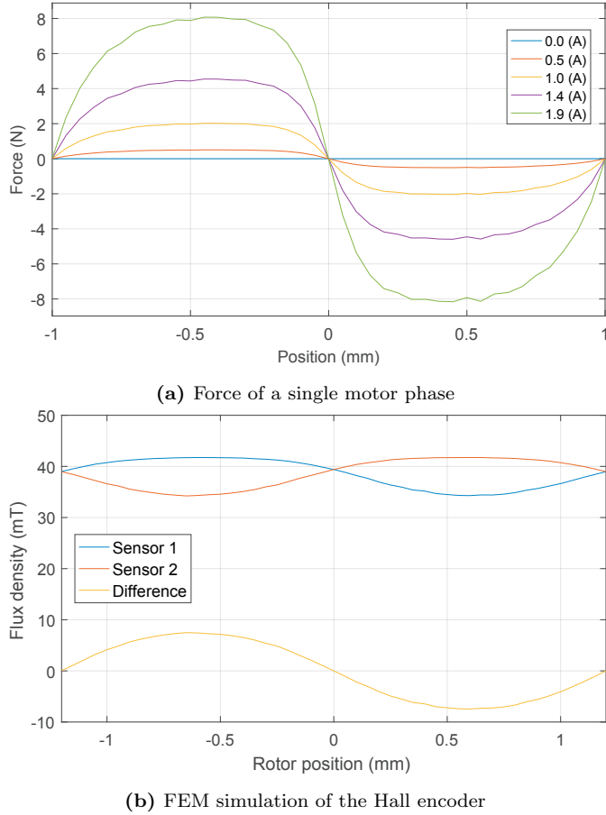
Fig. 3. FEM results for the force of a single motor phase with a limited number of rotor teeth (a) and for Hall sensor 1 and 2 for a static magnetic field of 40 mT (b).
