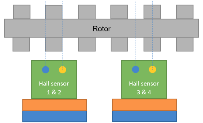
Fig. 4. Working principle of the Hall encoder.
