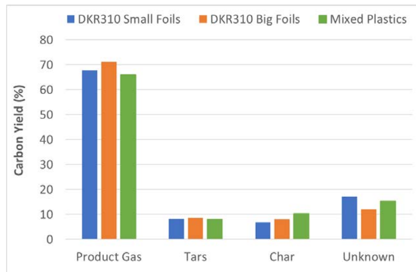
Figure 3.6: Carbon mass balance in the gasification of the plastic streams
