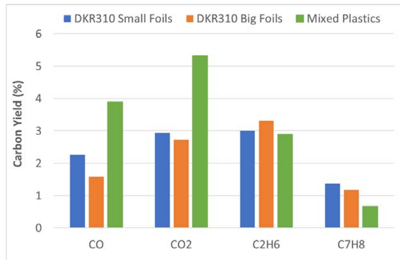
Figure 3.8: Carbon yield of some components present in the product gas from gasification of plastic waste streams
