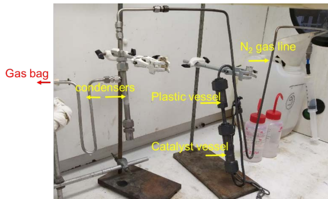
Figure 2.4: Picture of the gram-scale setup
