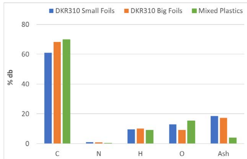
Figure 3.5: Feedstock analysis of the tested end-of-life plastic streams
