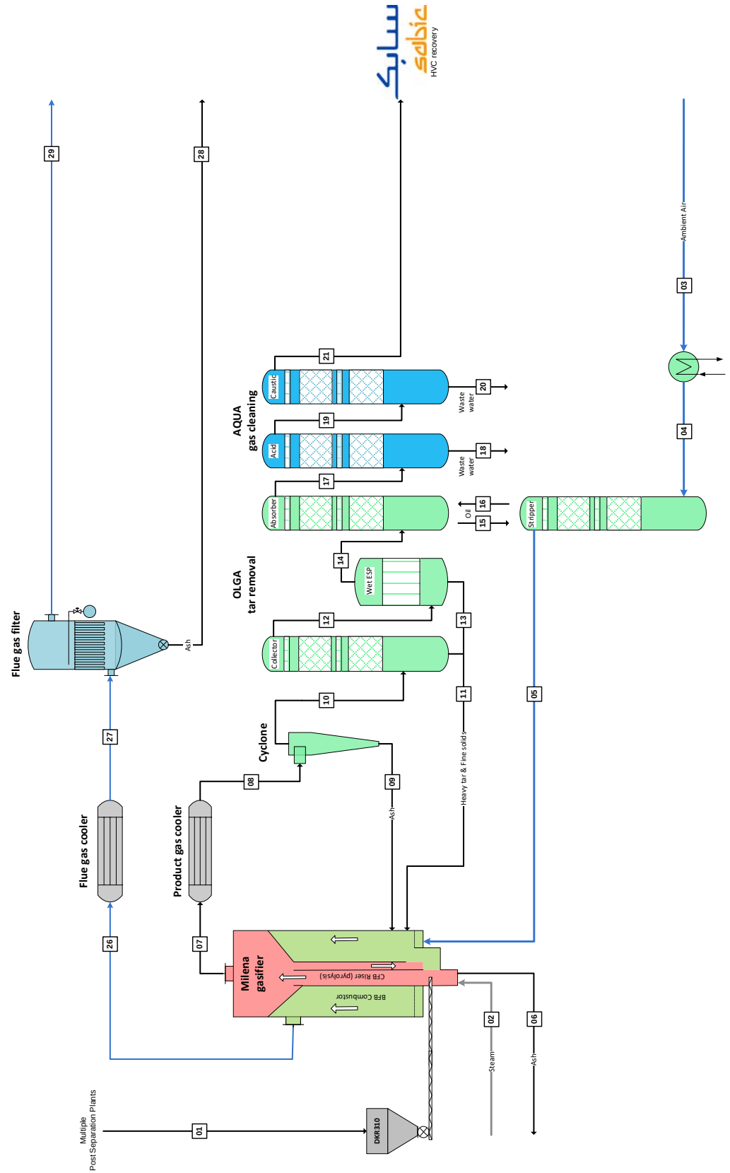
Figure 6.3: Process flow diagram of chemical recycling fitted into refinery setting
