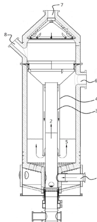
Figure 5.1 MILENA reactor
