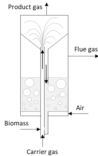
Figure 3.4: Scheme of the lab-scale Milena gasifier (25 kW th )
