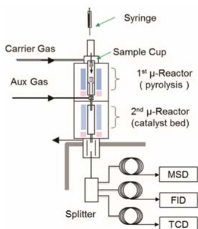
Figure 2.1: Schematic diagram of the micro-pyrolysis system
