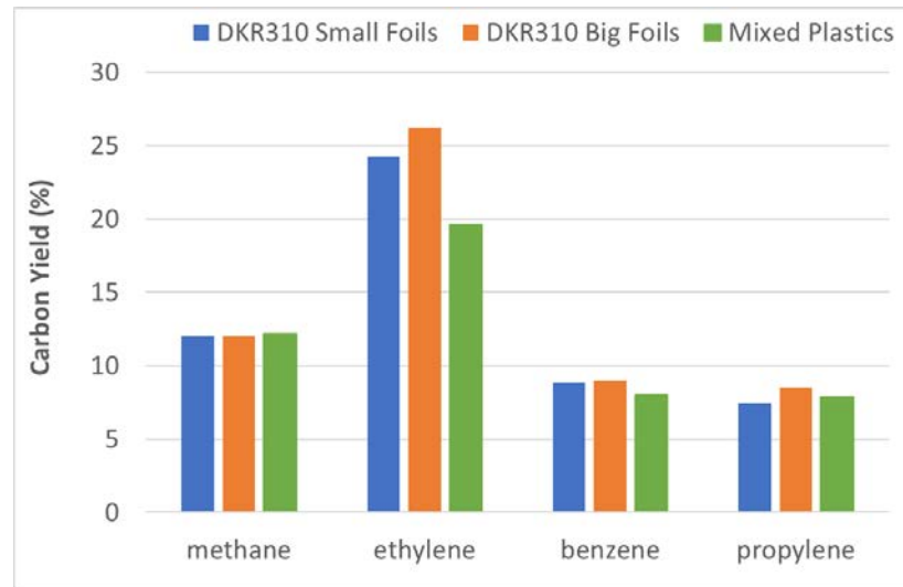
Figure 3.7: Carbon yield of some components present in the product gas from gasification of different plastics waste streams
