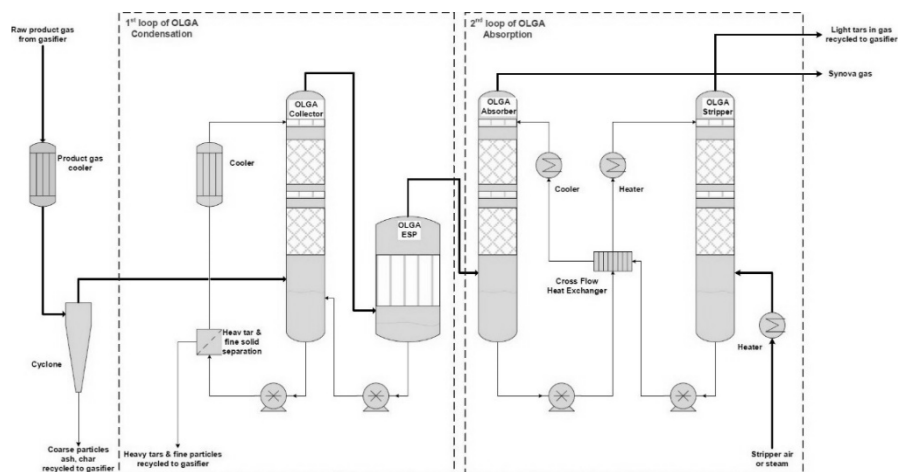
Figure 4.2: Scheme of the OLGA tar removal system
