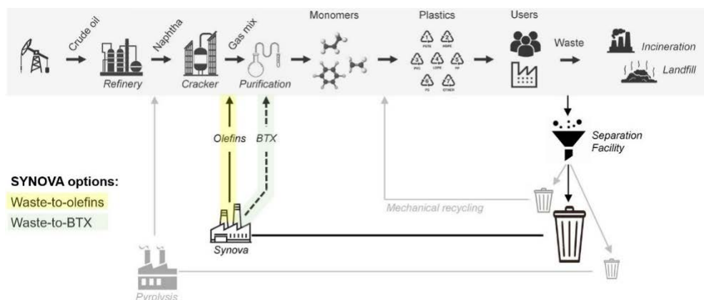
Figure 6.2: Process schemes of chemical recycling fitted into refinery setting
