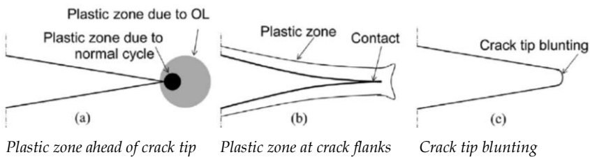
Figure 2: Schematic presentations of retardation concept (Maljaars et al., 2015)
