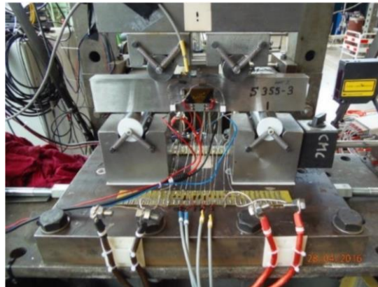
Figure 22: Side view of the SENB4 specimen, including instrumentation
