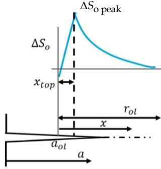
Figure 9: Schematic representation of the change in \Delta S_{0k} after an OL applied at a_{OL}
