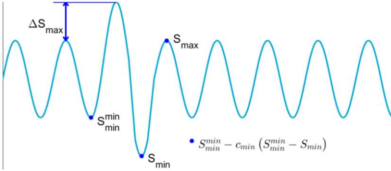
Figure 15: Schematic overview of an OL / UL combination and the correction of S_{\min}^{\min}
