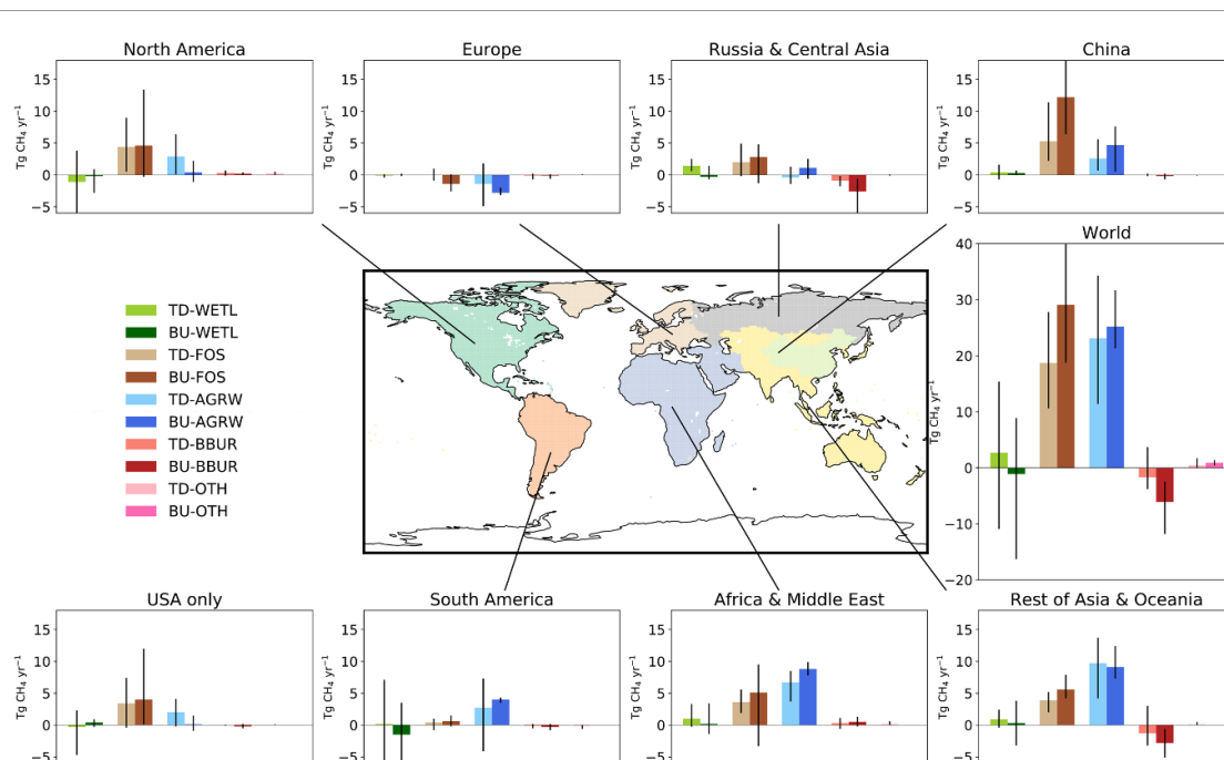
Figure 4. Changes in methane emissions ( \text{Tg CH}_4 \text{ yr}^{-1} ; min-max range) by region and source for year 2017 compared with the mean annual value for the period 2000–2006. Positive values represent annual emissions that were larger in 2017. Abbreviations in the color legend refer to top-down (TD) and bottom-up (BU) methods and to ‘wetland,’ ‘fossil,’ ‘agriculture and waste,’ ‘biomass burning,’ and ‘other’ sources. See section 1 and the figure 3 legend for descriptions of max-min ranges across inventories, models, and products.
