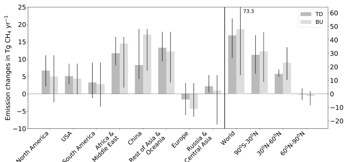
Figure 3. Changes in total methane emissions (mean and min-max range in \text{Tg CH}_4 \text{ yr}^{-1} ) in 2017 compared with mean values for 2000–2006 by region (left panel) and latitude (right panel; note different y -axis scales). Each pair of bars presents top-down (dark gray) and bottom-up (light gray) emissions estimates. See the figure 2 legend for a map of the regions. Positive values reflect emissions that were larger in 2017 than in the period 2000–2006. For top-down (TD) estimates, the mean, minimum and maximum values correspond to values across the ensemble of 11 model inversions. For bottom-up (BU) estimates, they are the mean, min and max values of the total emissions ensemble obtained by combining 4 anthropogenic inventories with 3 fire products and 13 wetland emissions model results.
