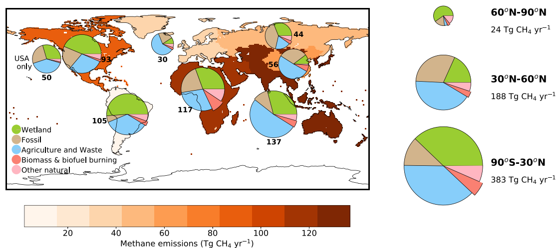
Figure 2. Methane emissions (Tg CH 4 yr -1 ) for 2017 by region, source category, and latitude. The mean estimates shown arise from the ensemble of top-down inversion models described in Saunio et al (2020).
