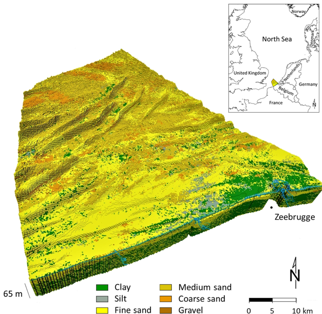
Fig. 1. View of the subsurface voxel model for the Belgian part of the North Sea (BPNS) (Hademenos et al. 2018).
