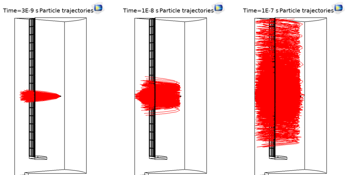
Figure 6. Electron trajectories after release from the filament. Three different release times: 3 ns (left, just before the electrons have reached the center axis), 10 ns (middle, just before the electrons have reached the center axis for the second time) and 100 ns (right).
