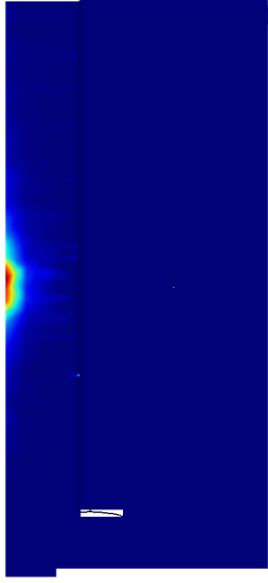
Figure 7. Electron space charge density inside anode cage indicating ionization sites.
