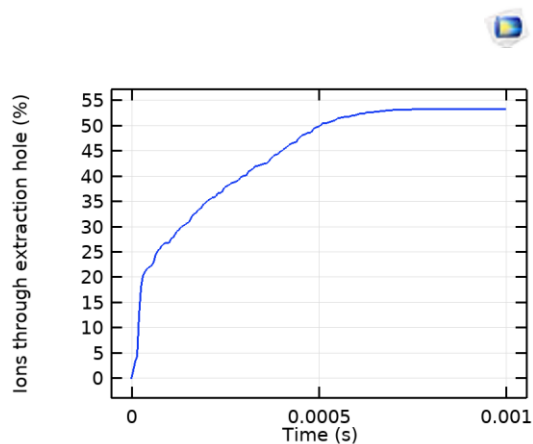
Figure 11. Ions collected at extraction hole.
