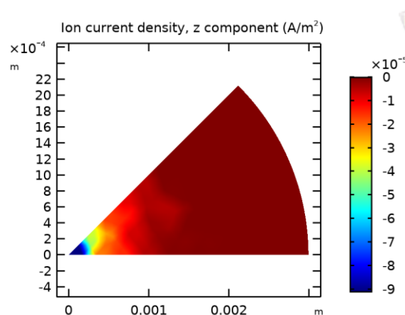
Figure 12. Ion beam intensity at the extraction hole.
