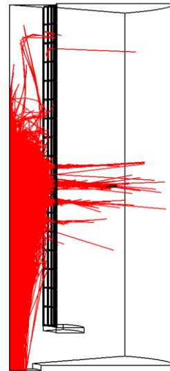
Figure 10. Ion trajectories after ionization.
