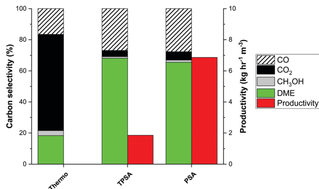
Fig. 2 Thermodynamic (maximally possible) carbon distribution without sorption enhancement versus experimentally obtained TPSA and PSA results for sorption enhanced DME synthesis. Conditions: 275 °C and 25 bar for a CO 2 :CO = 2:1 feed with stoichiometric hydrogen and CH 4 tracer. TPSA: regeneration included heating up to 400 °C.
