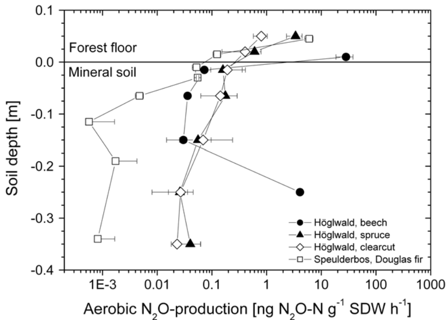
Fig. 4. N 2 O production in different soil depths and at different sites under aerobic incubation conditions. Given are mean values \pm SE.
