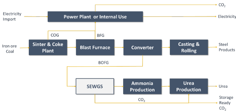
Figure 3. BOF2UREA Plant
