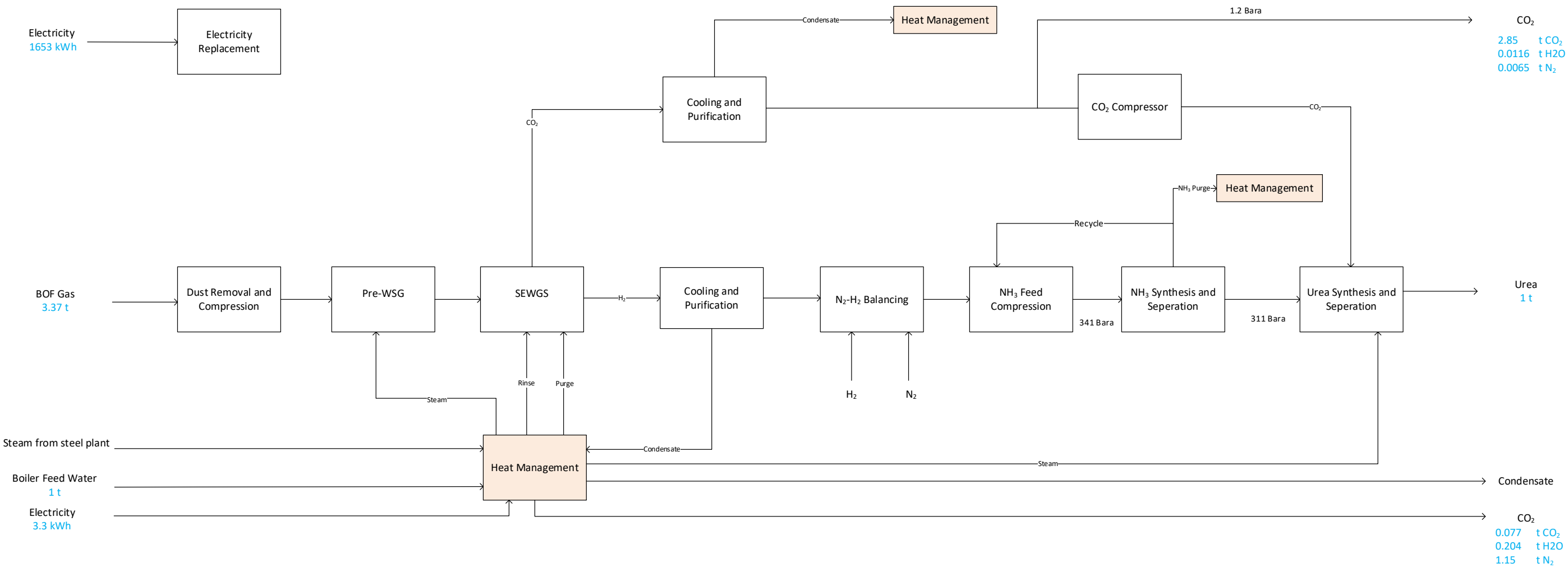
Figure 5. Process Flow Diagram for BOF2UREA
