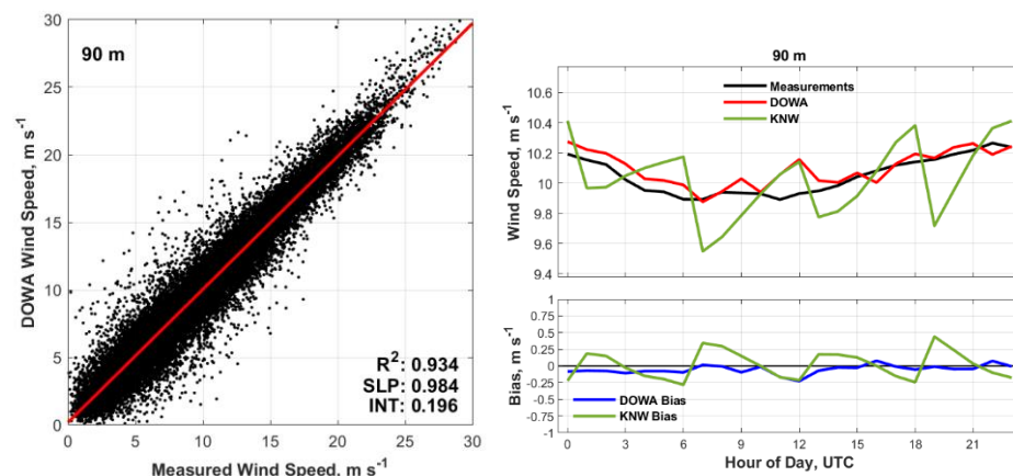
Figure 5: Left: Scatter plot of DOWA wind speeds against MMIJ wind speeds at 90m. Right: Hourly mean wind speeds (top) and bias (bottom). Bias = measured – atlas.
