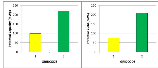
Figure 3: Potential capacity in MWp and expected yield in GWh of the optimally suitable areas (Grid code 2) and partially suited areas (Grid code 1)
