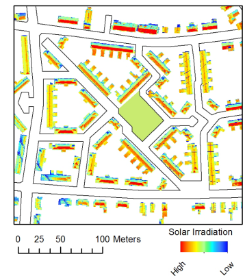
Figure 3: Solar Irradiation image derived for building by running the Solar Radiation tool. South facing slopes are seen to receive greater irradiation.
