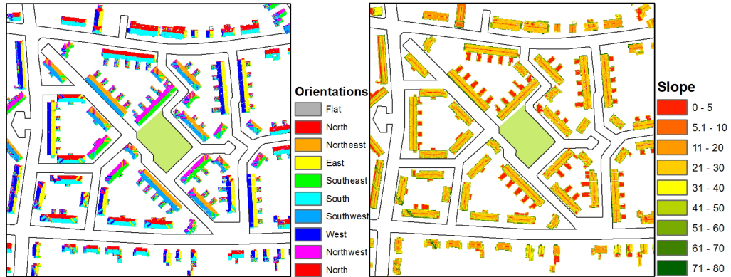
Figure 4: Left: Orientation image showing the direction of slope of the rooftops. Right: Slope image classified in classes to distinguish between flat and sloping roofs.
