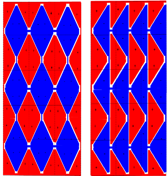
Figure 4: Contacts at the rear of the MWT cell. An extra contact is to allow bridging the crossings and examples of the interconnections in the foil for the bridge-foil concept
