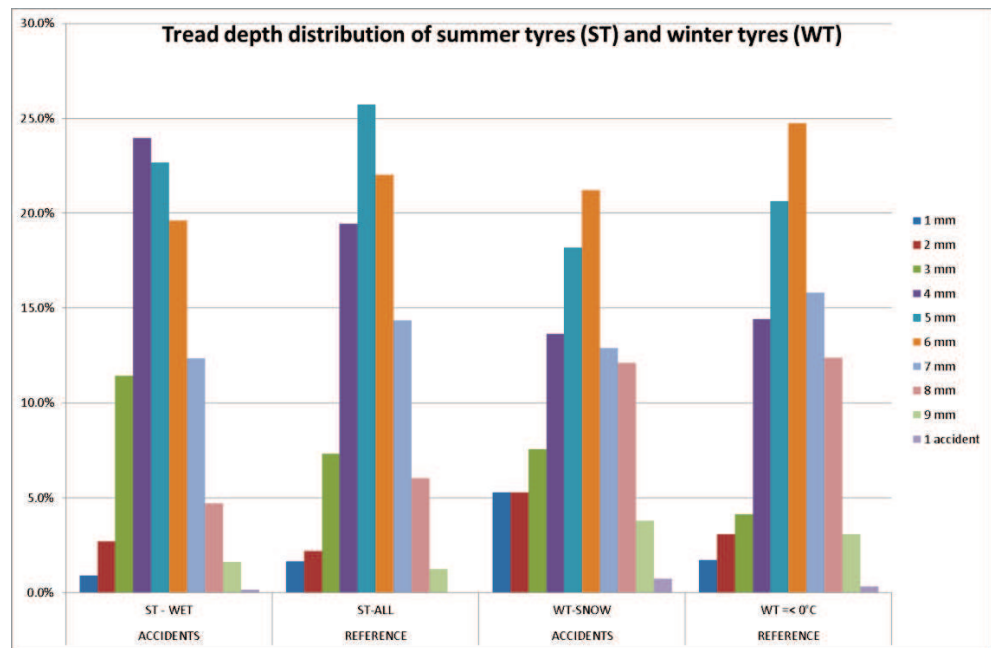
Figure 4.5: Tread depth distribution in accidents on wet roads (Summer tyres) and snow (Winter tyres).
