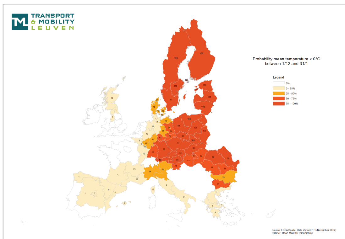
Figure 3.10: Probability of mean temperature &lt;0°C between 1-12 and 31-01.
