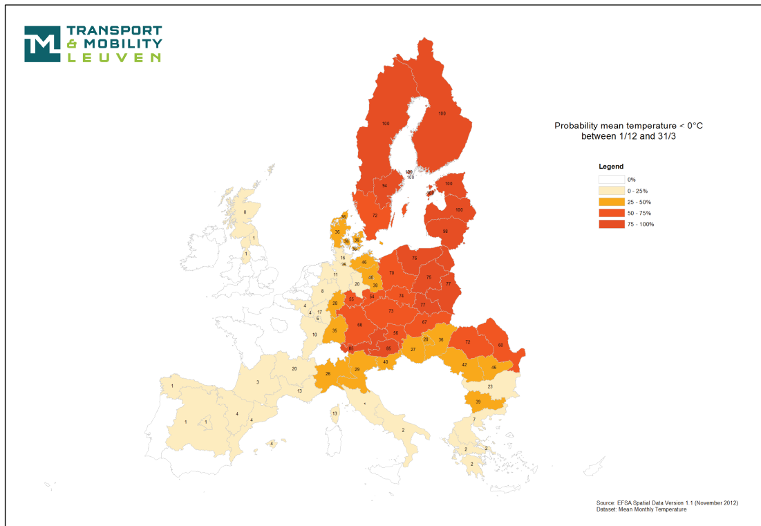
Figure 3.12: Probability of mean temperature &lt;0°C between 1-12 and 31-03.
