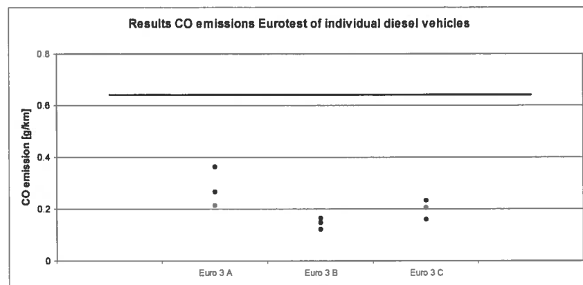
Figure 14: CO-emission of individual diesel vehicles
