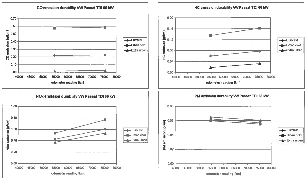
Figure 38 Emissions over the lifetime of a Volkswagen Passat TDI 66 kW
