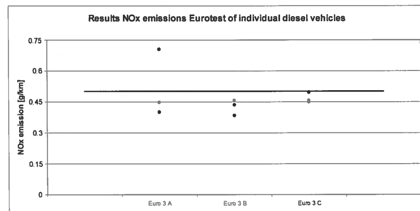
Figure 16: NO x -emission of individual diesel vehicles
