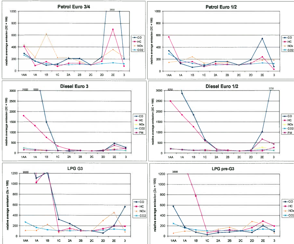
Figure 32: Relative average emission profiles of all separate vehicle categories (2C is 100%)
