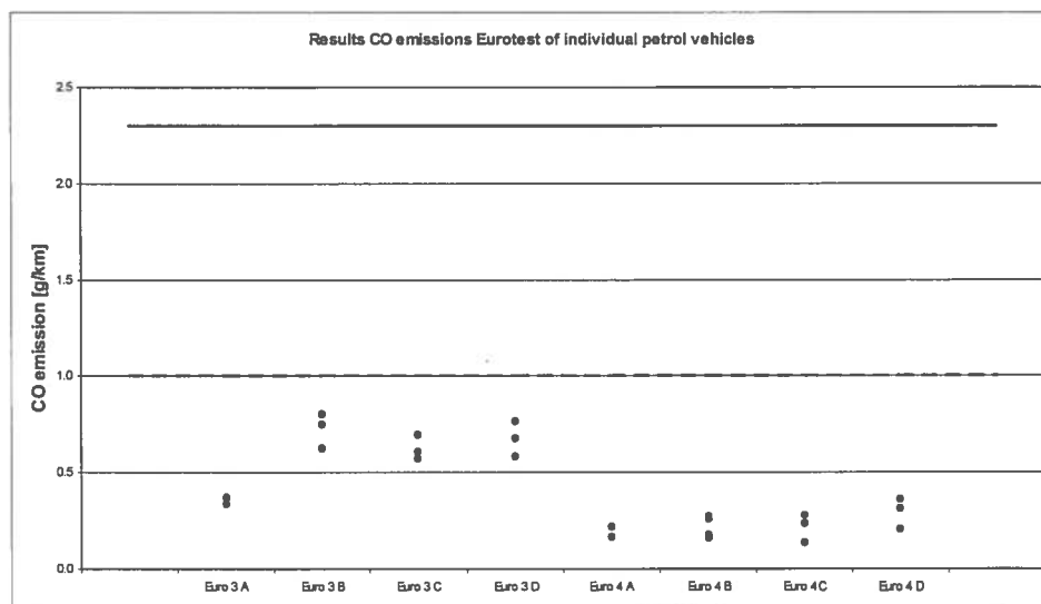
Figure 3: CO-emission of individual petrol vehicles
