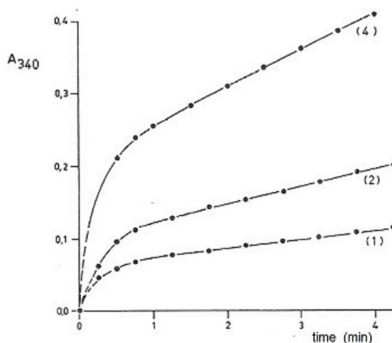
Fig 6.8 Effect of tropic acid and \text{NAD}^+ concentration
