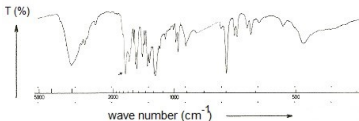
Fig 3.3 Infra-red spectrum of pma in carbon tetrachloride X-axis: wavenumber ( \text{cm}^{-1} ); Y axis: transmission T (%)
