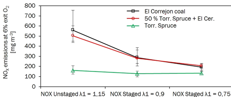
Fig. 8. Impact of air staging at primary \lambda_1 0.9 and 0.75. NO x emissions during El Correjón coal and torrefied spruce (co)firing in down-fired 500 kW pilot scale plant.
