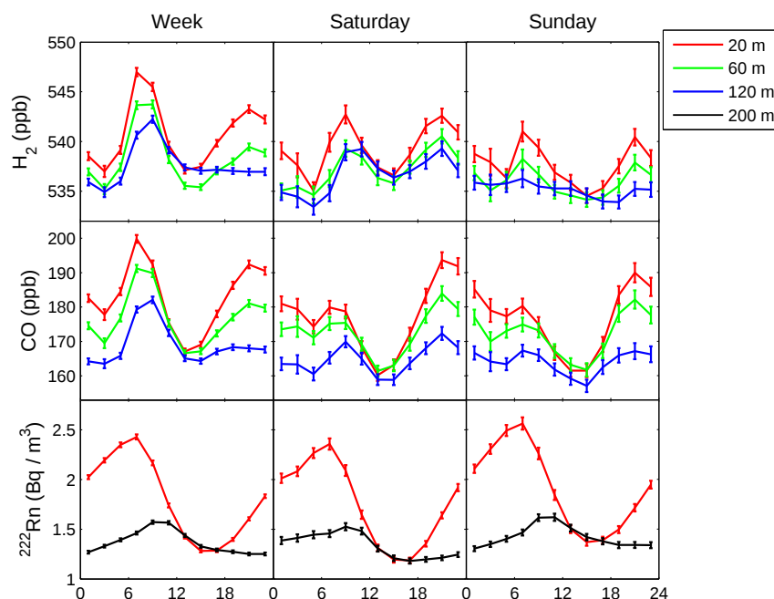
Fig. 7. Average diurnal cycles of H_2 , CO and ^{222}\text{Rn} , for weekdays, Saturdays and Sundays. Each data point is the trimmed average (discarding the 10% lowest and highest values) of a 2-hourly bin. The data between 03:00 and 04:00 were excluded, because the daily calibration took place mostly during this interval, thus the results were possibly biased. For H_2 and CO, the data from the 200m height are not shown for the reason explained in Sect. 3. The error bars are standard errors of the means corresponding to 67% confidence intervals.
