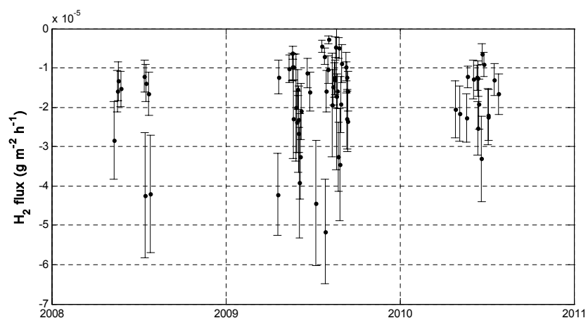
Fig. 8. H_2 soil deposition flux calculated with the ^{222}\text{Rn} tracer method for selected deposition events.
