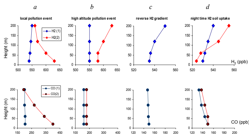
Fig. 6. Vertical profiles of H_2 (top) and CO (bottom) for various atmospheric situations. Except for plots (c), vertical profiles before (blue) and during the event (red) are shown (see text for explanations). Note that the x-axis ranges are not the same for all plots, but the proportion between H_2 and CO ranges is maintained.
