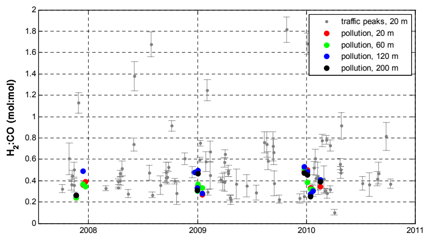
Fig. 10. H_2/CO ratios of large scale pollution events, for the four sampling heights. Overlapped are the ratios of the morning traffic peaks, for comparison. The results are not corrected for the concurrent soil uptake.
