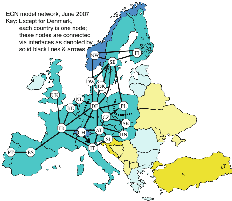
Fig. 1 Representation of the electricity network in COMPETES ( dashed lines represent constraints on the sum of flows on the links shown)
