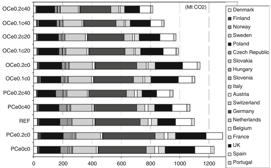
Fig. 6 Total CO 2 emissions of the power sector in the EU-20 under various COMPETES model scenarios (REF case is equivalent to PCe0c20 and PCe0.2c20.)
