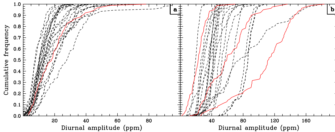
Figure 5. Cumulative frequency distribution for the peak-to-peak diurnal amplitude for June to August of observed CO 2 (red) and modeled CO 2 (black) for (a) BOR and (b) TPJ. At TPJ the observations are for 62 m (left line), 29 m (center line), and 20 m (right line).
