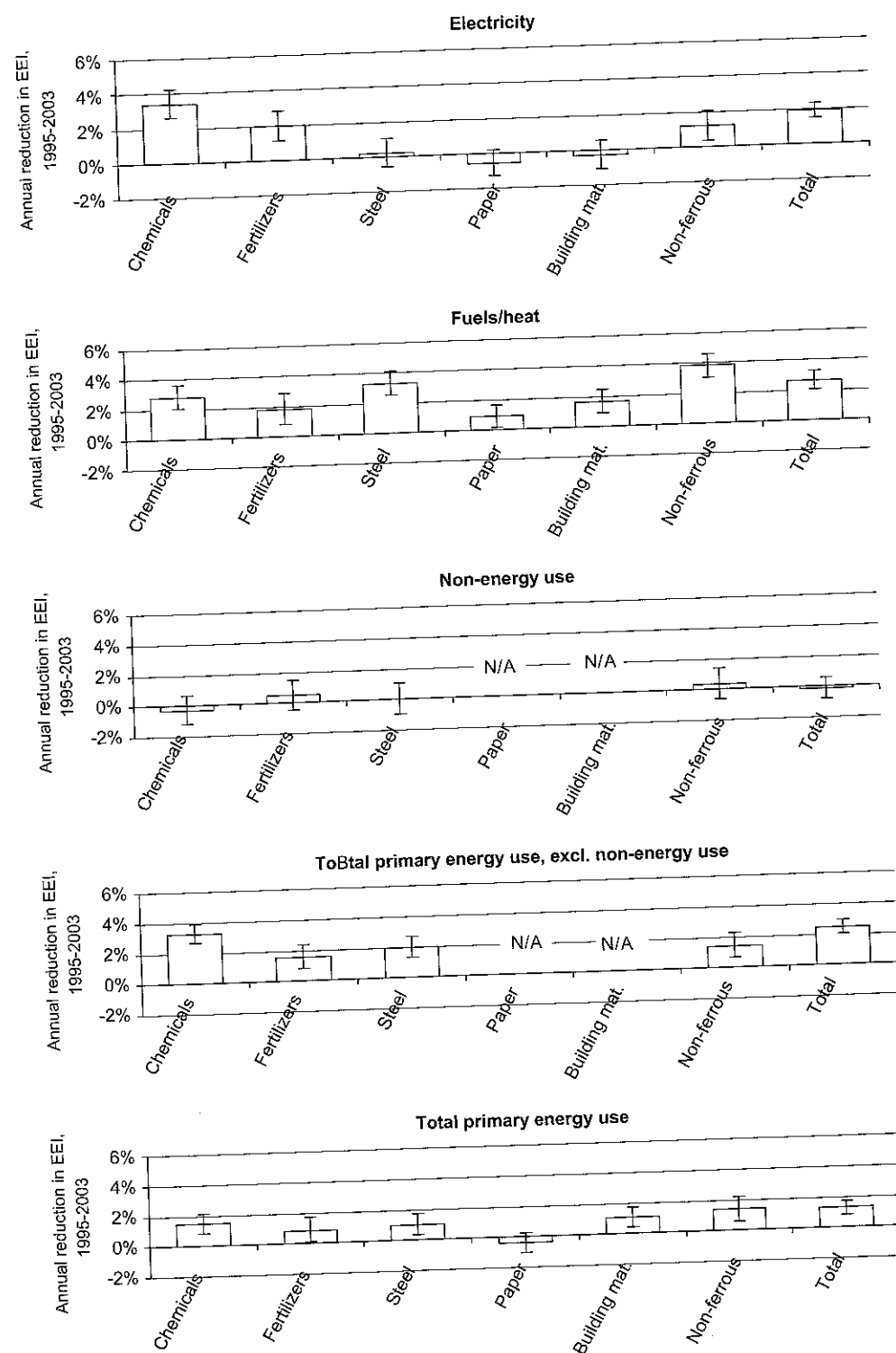
Fig. 1. Annual reduction in EEI between 1995 and 2003 (%/year).
