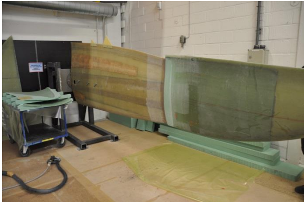
Figure 5-12: Glued tip pre- and post-grinding
