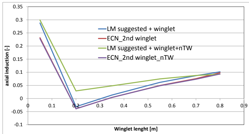
Figure 4-14: Axial induction on the winglet
