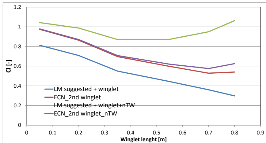
Figure 4-15: Cl on the winglet
