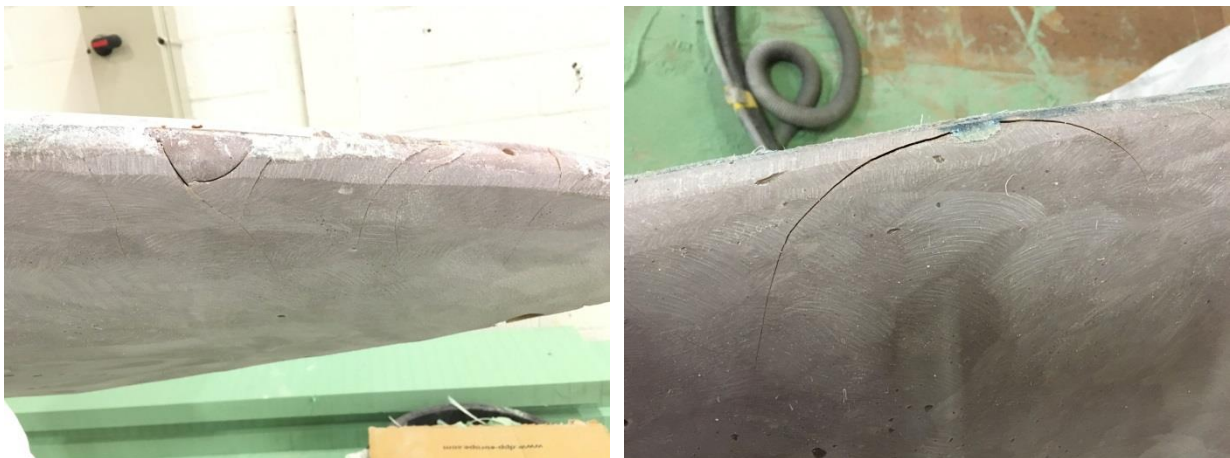
Figure 5-23: Glue cracking as seen after extreme load test
