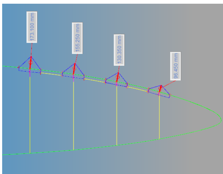
Figure 4-35: Final turbulator configuration applied to the blades of the test wind turbine
