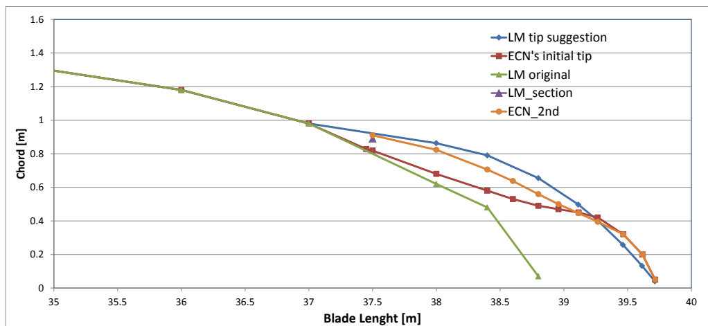
Figure 4-7: Tip chord variations and alternatives including the constrained chord length (purple triangle)
