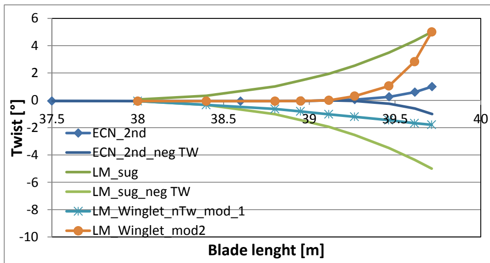
Figure 4-8: Twist variations and alternatives both for the conventional tip and the winglet
