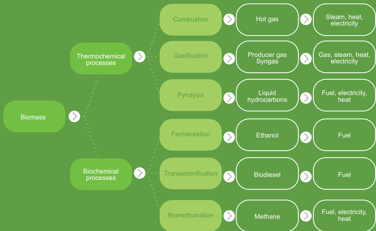
Figure 7: Broad categorisation of biomass conversion processes
