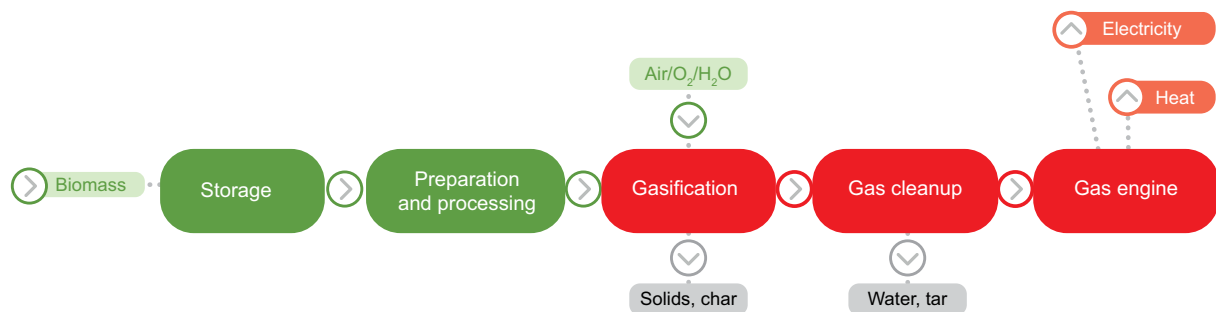
Figure 16: Block flow diagram of biomass gasification for electricity generation and heat recovery via CHP
