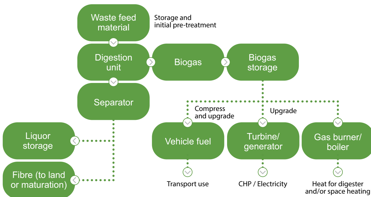
Figure 13: Anaerobic digestion as a means to produce energy and fertiliser (SSWM 2013)
