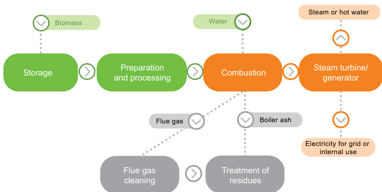
Figure 8: Block flow diagram of the process for electricity generation from biomass via combustion
