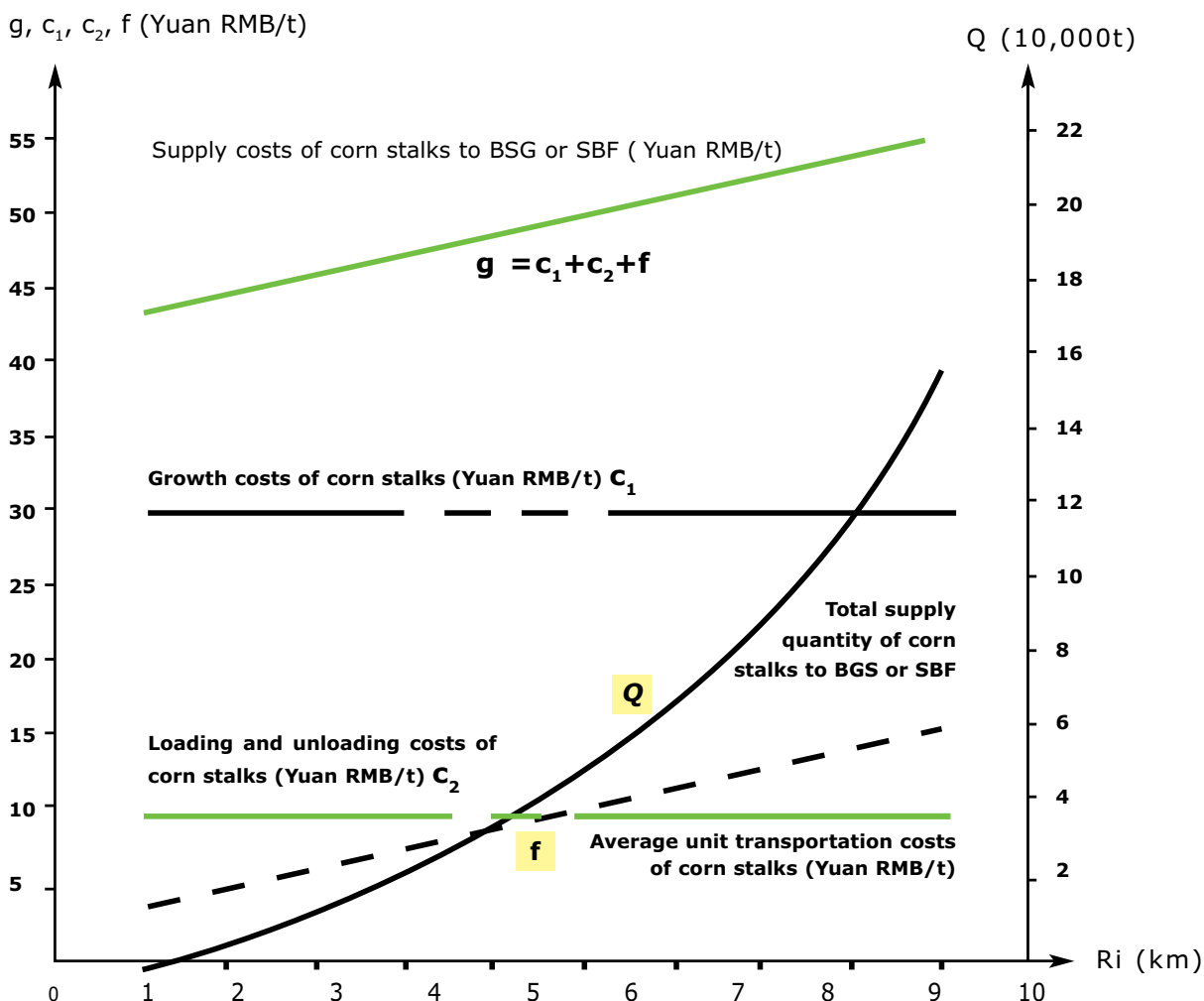
Figure 23: Example of a detailed analysis of quantity and cost of corn stalks in a province in China showing transport costs (Cai 1998 in UNDP 2000)
