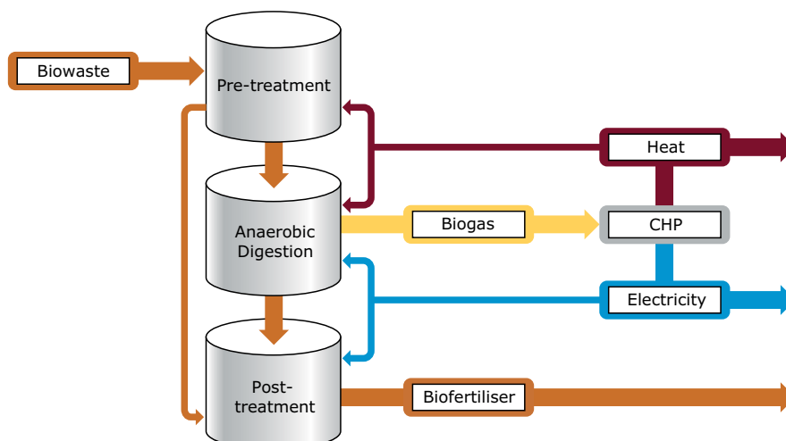
Figure 11: Example of a biogas plant configured to produce energy and fertiliser from waste feedstock (DEFRA 2011)
