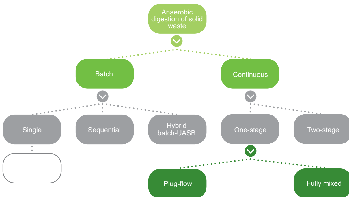
Figure 12: Process configurations for anaerobic digestion of solid waste (Angelidaki et al. 2011)
