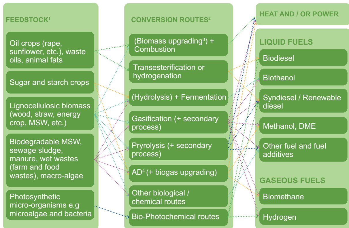
Figure 22: Schematic view of the wide variety of bioenergy routes (IEA 2009)
