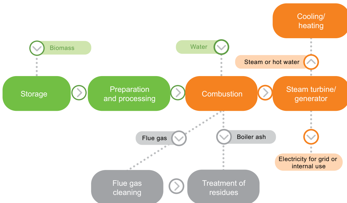
Figure 9: Block flow diagram of the process for electricity generation and heat recovery via CHP
