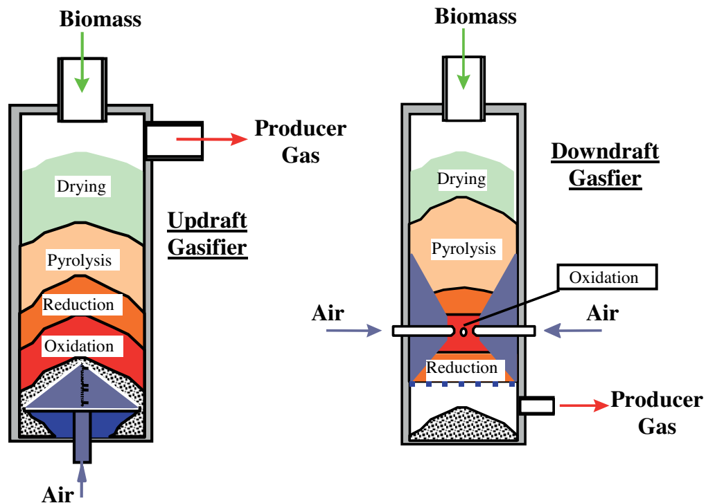
Figure 14: Schematic comparison of updraft and downdraft gasification (van der Meijden 2010)
