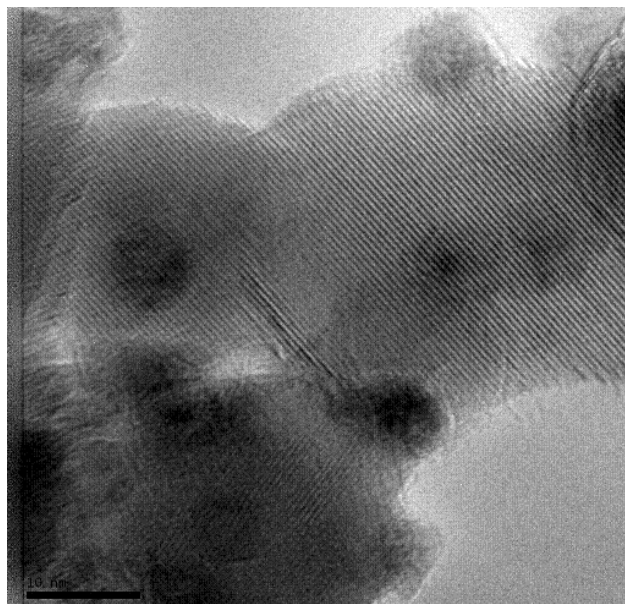
Figure 1: Microscopic image of a supported Nickel – Boron catalyst. The nickel particles are visible as darker spots, sizing up to 7 nm
