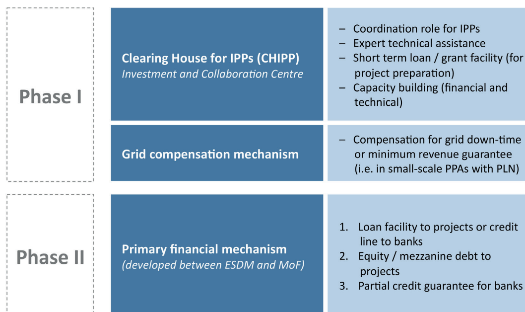
Figure X1: NAMA components
