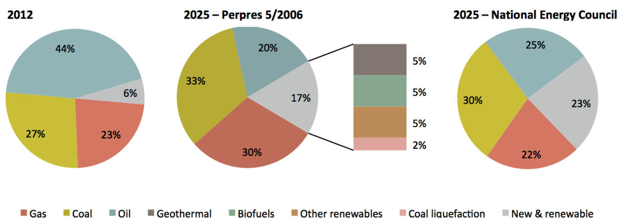
Figure 3: Primary energy mix, excluding biomass, in 2012 and 2025 under two scenarios (source: Gol 2006; Lubis 2013; ESDM 2014a)
