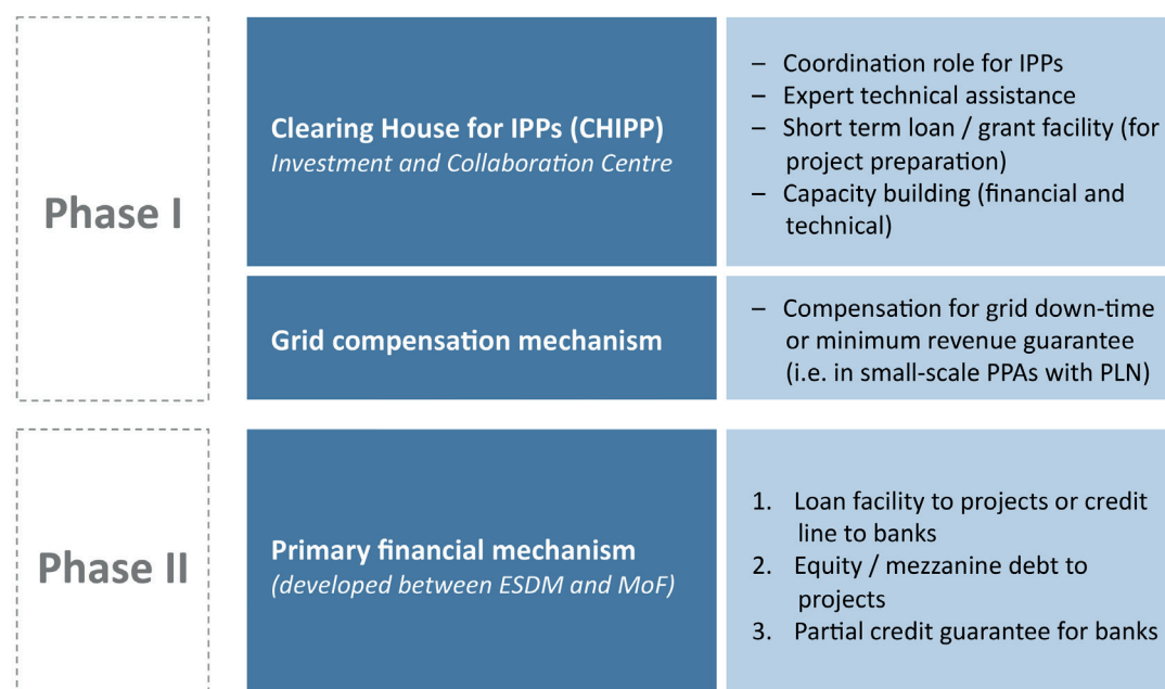
Figure 9: NAMA components
