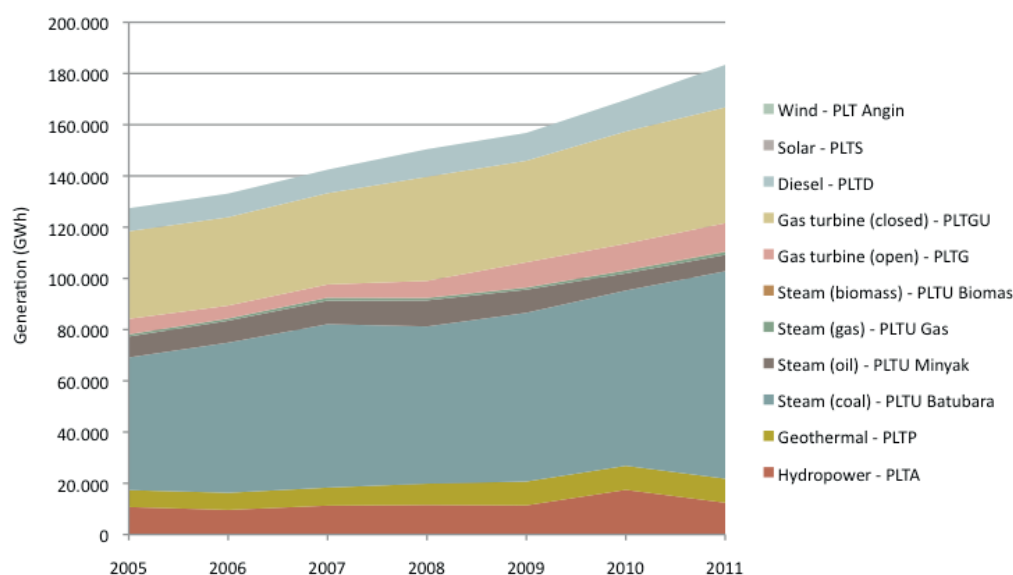
Figure 2: Electricity generation by source 2005 - 2011 (source: ESDM 2013)
