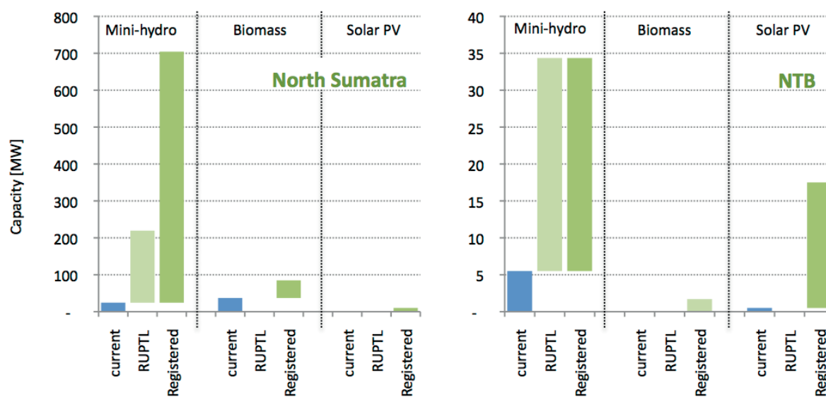
Figure 8: Current, PLN planned and registered capacities for mini-hydro, biomass and solar PV in two pilot provinces; North Sumatra [left] and NTB [right] (source: own derivation from sources in Table 5)
