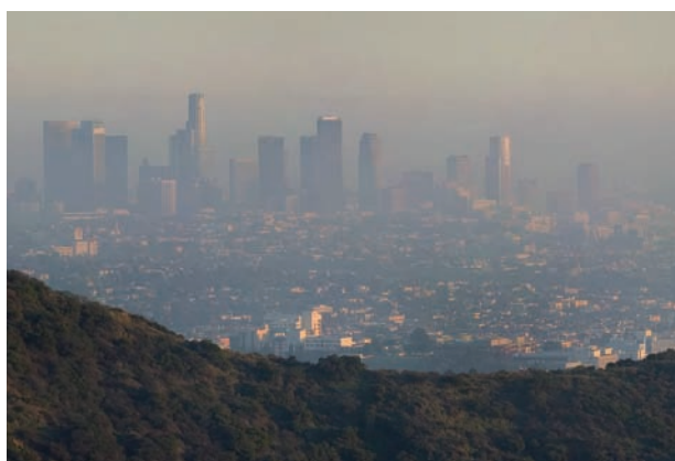
Figure 4.4 Images of poor air quality. The pollution haze indicates high levels of particulate matter, much of which originates from N pollution, including particulate matter containing ammonium and nitrate, and high levels of nitrogen oxides ( NO_x ). Left: Los Angeles, US (Photo: DAVID ILIFF. License: CC-BY-SA 3.0). Right: Santiago, Chile (Photo: Michael Ertel).
