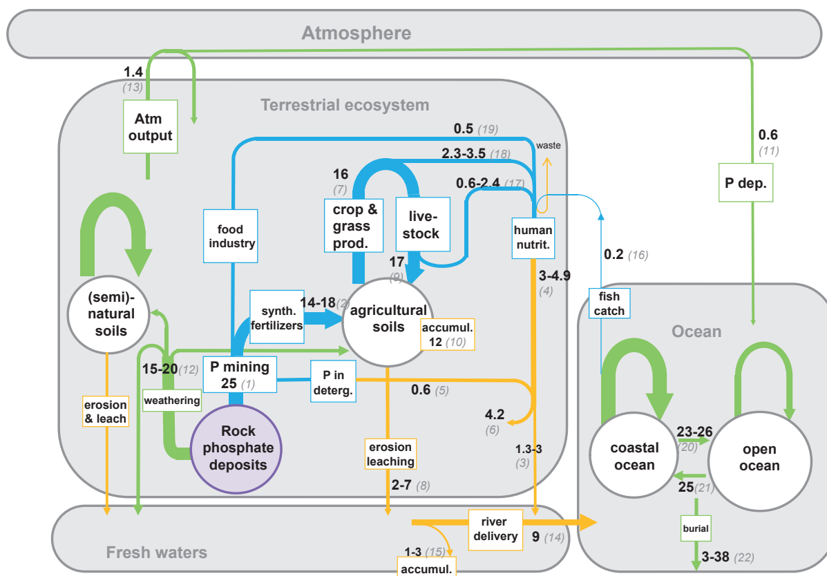
Figure 3.2 Global phosphorus cycle around the years 2000-2010. The arrows show the phosphorus fluxes across environmental pools and compartments ( green : natural fluxes, blue : intended fluxes, orange : unintended fluxes or substantially perturbed fluxes, more explanation is provided in the text). The figures in black indicate the phosphorus fluxes in Tg P per year and the figures within brackets are the legend and refer to the accompanying table including the references for each flux (see Table 3.2). Note that not all figures add exactly, due to the use of different data sources.
