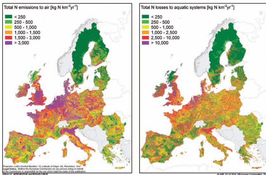
Figure 7.3 Estimated distribution of reactive nitrogen emissions across Europe (expressed as \text{kg N} per \text{km}^2 for 2000) including (left) emissions to air as the sum of \text{NO}_x , \text{NH}_3 and \text{N}_2\text{O} , and (right) total losses to aquatic systems, including nitrate and other \text{N}_r leaching and wastewaters. These high spatial resolution maps illustrate the challenge of managing nitrogen flows given the wide spatial variation experienced (based on Leip et al., 2011).
