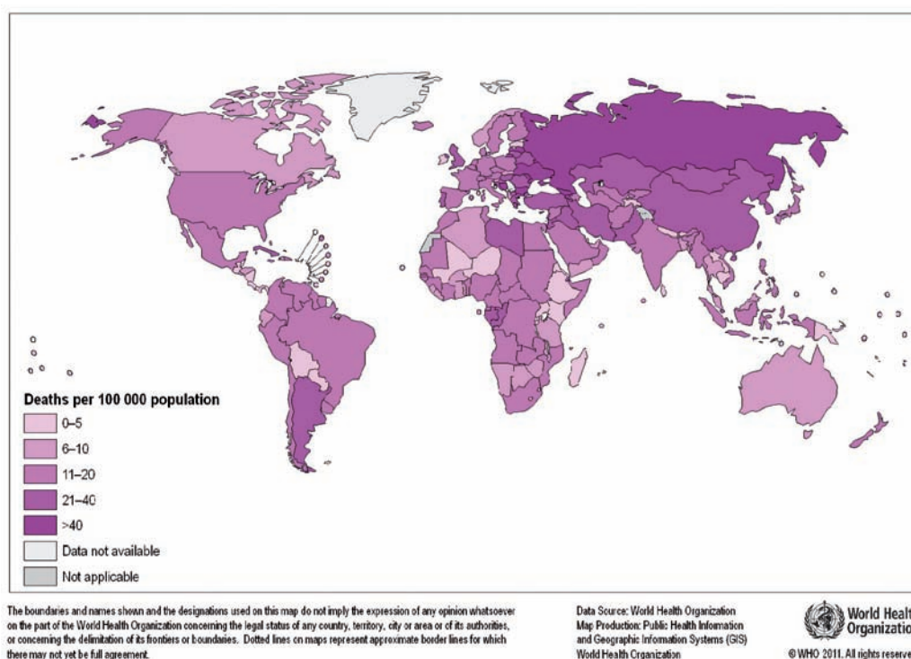
Figure 4.5 Deaths attributable annually to outdoor air pollution in 2008 (WHO, 2011), incorporating contributions from reactive N emissions (through effects on particulate matter, tropospheric ozone and nitrogen dioxide).
