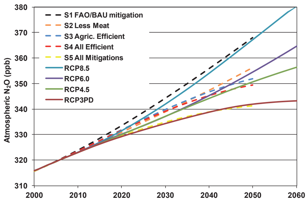
Figure 3.5 Projected atmospheric N_2O concentrations for the four IPCC-AR5 representative concentration pathways (RCPs) and the five scenarios from Davidson (2012): S1 = FAO population and dietary projections (FAO, 2006) with no new N_2O mitigation efforts; S2 = same as S1 but also 50% reduction in mean per capita meat consumption in the developed world by 2030 relative to 1980 consumption; S3 = same as S1 but improvements in agricultural efficiencies that reduce N_2O emissions factors for N mineral fertilizers and manure by 50% by 2050; S4 = same as S3 but also 50% emission reductions in industry and transportation sectors and by biomass burning; S5 = combination of S2 and S4.
