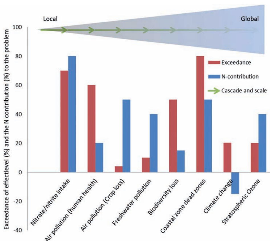
Figure 4.13 Comparison of exceedances of environmental threats related to \text{N}_r and the contribution of \text{N}_r to each of these threats compared with other drivers. While the approach recognizes that some effects are local and some global, values represent global estimates (Erismann et al., 2013).
