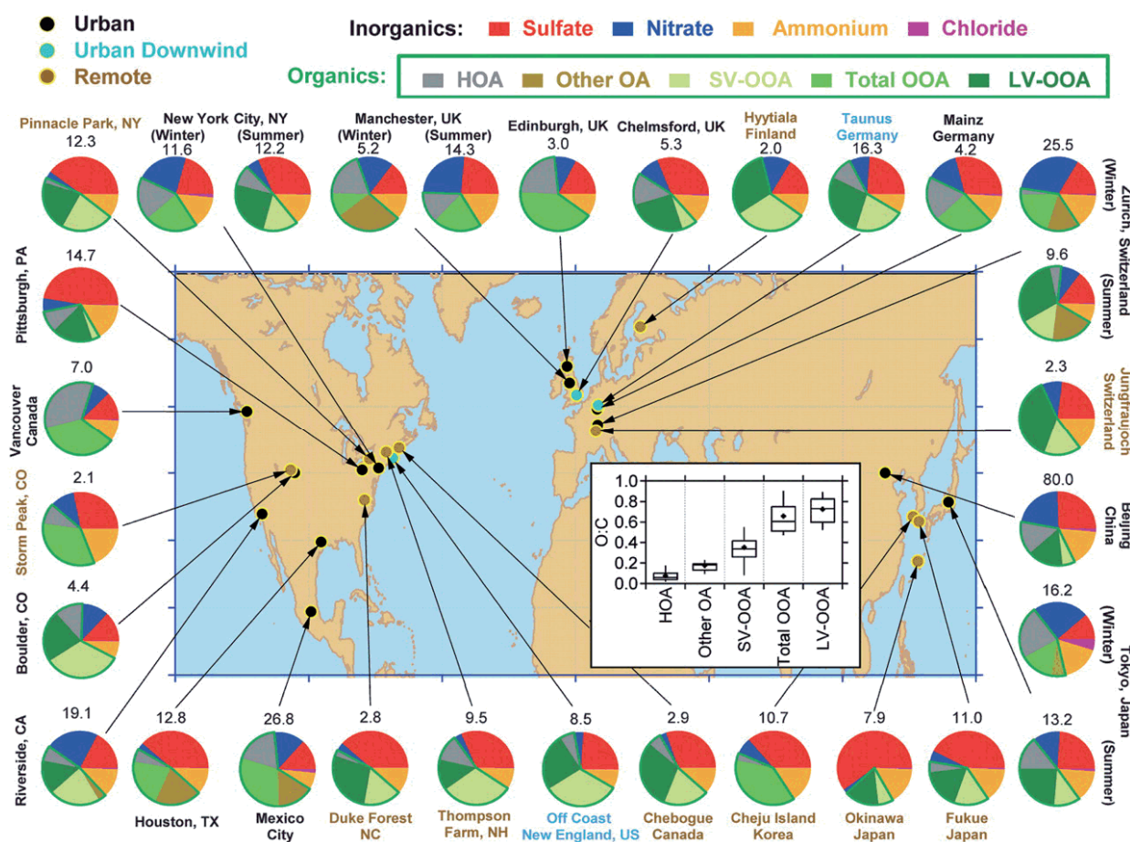
Figure 4.6 Contribution of nitrogen compounds to fine particulate matter in different locations around the world. Results of measurements using aerosol mass spectrometry (less than 1 \mu m size, PM_{10} ), with the N_r fraction represented by nitrate (blue) and ammonium (orange) (Jimenez et al., 2009). The organic aerosol (OA), are distinguished into different fractions of hydrocarbon-like organic aerosol (HOA) and oxygenated organic aerosol (OOA), including low volatility (LV) and semi-volatile (SV) fractions.
