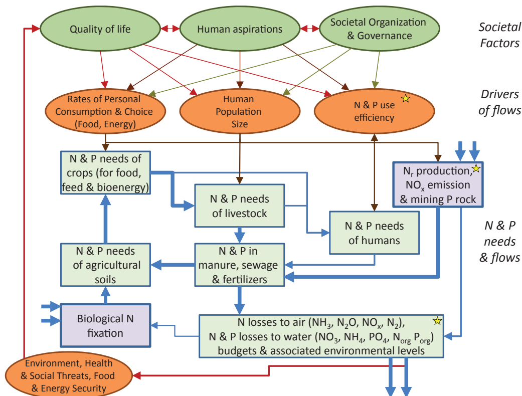
Figure 4.12 Conceptual diagram of nitrogen (N) and phosphorus (P) cycles in relation to societal factors and drivers (green and brown), needs and flows (blue) in relation to the development of 'planetary boundaries' to indicate thresholds for adverse effects, which should be considered in relation to the meeting of basic social needs. ★, indicates some possible points for setting planetary boundaries (e.g., pollution losses and concentrations) and performance indicators (e.g., nutrient use efficiency, balance from calculating nutrient budgets) (original graphic).
