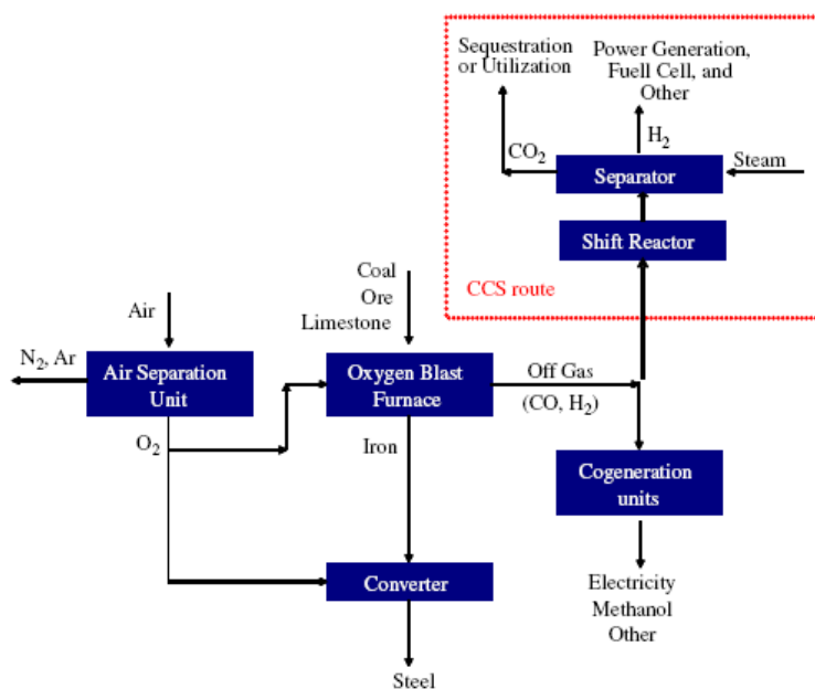
Fig. 14. Schematic view of P-OBF.
