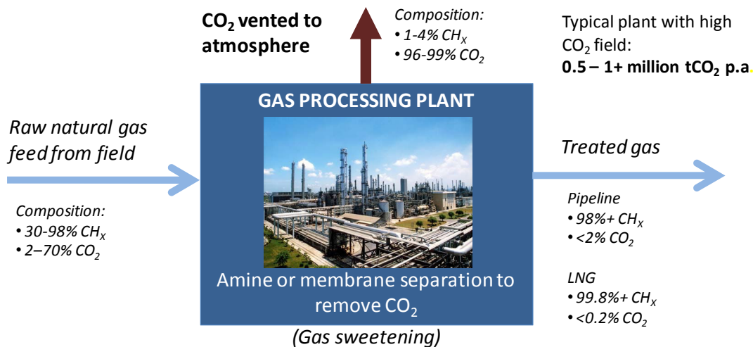
Figure 3.2 Natural gas sweetening configuration
