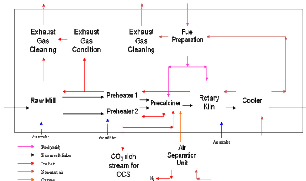
Figure 3.7 Process diagram of a partial capture oxyfuel cement plant design
