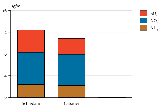
Average concentrations of NH 4 , NO 3 and SO 4 in PM 10 (MARGA) at the three locations
