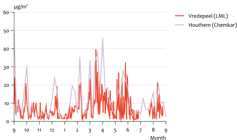
Time series of SIA for Vredepeel (LML) and Houthem (rural background location in Chemkar).
