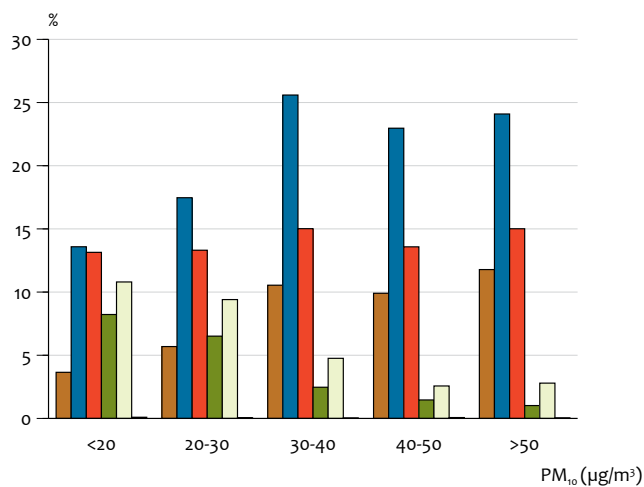
Relative distributions of the various components as a function of PM concentration classes at Cabauw and Schiedam.
