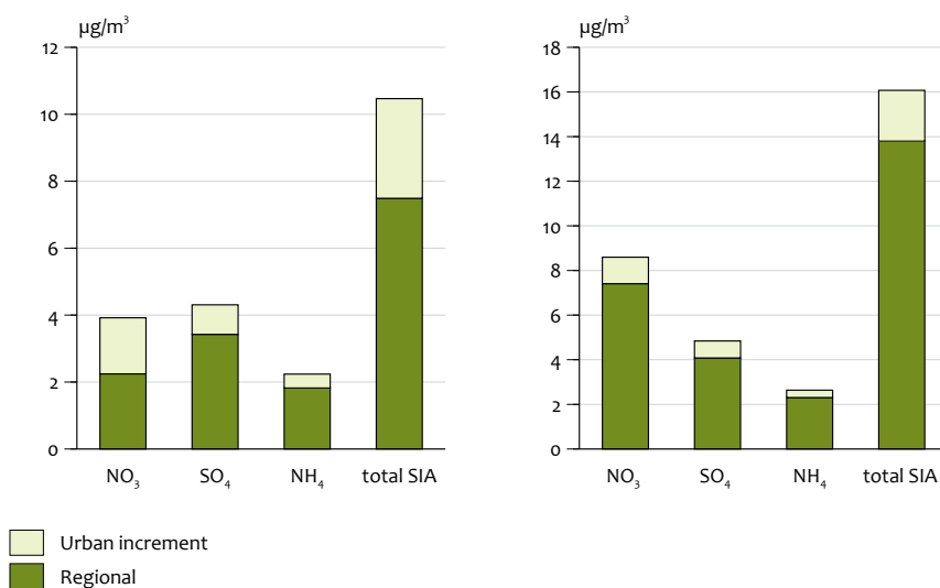
SIA concentrations in the IUTA (Germany) and Chemkar (Belgium) data sets.
