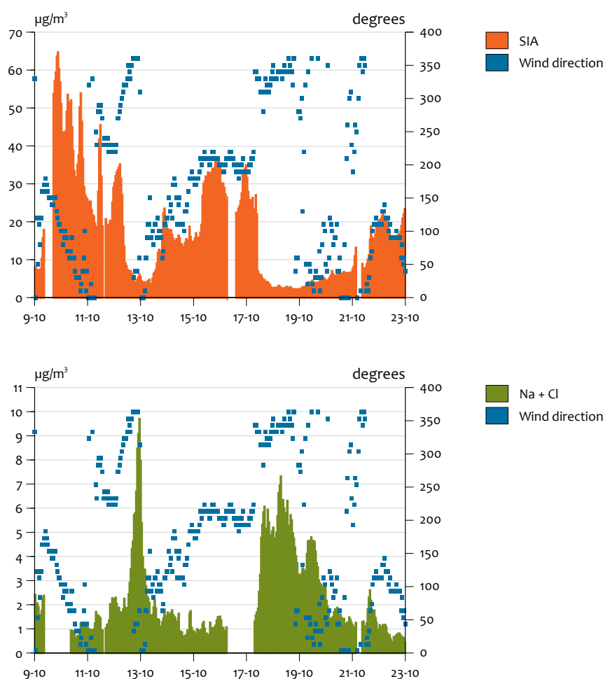
Hourly registrations of SIA and sea salt by the MARGA system in Schiedam.
