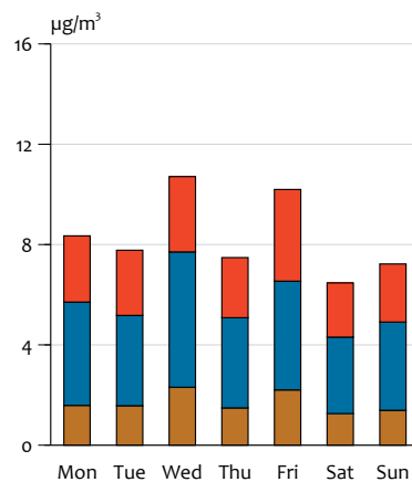
\text{PM}_{2.5} daily averages
