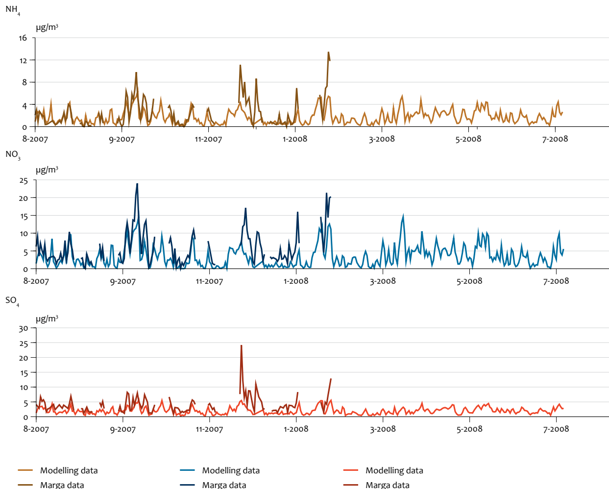
Time series of the modelling data and MARGA data for Schiedam..
