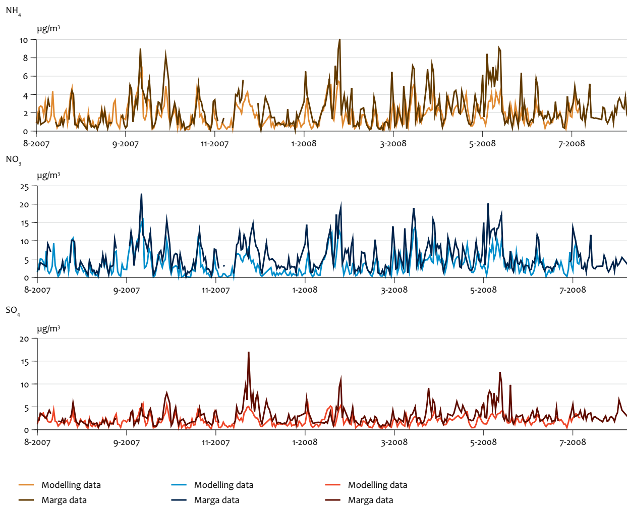
Time series of the modelling data and measured MARGA data for Cabauw.
