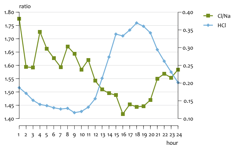
Daily cycles of Cl/Na and HCl, as measured with the MARGA system at Schiedam.
