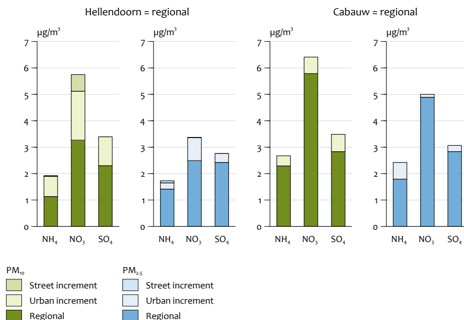
Incremental concentrations of ammonium, nitrate and anthropogenic sulphate, at the urban background location (Schiedam) and at the traffic location (Rotterdam), compared to the regional concentration levels at Hellendoorn (left) and Cabauw (right).
