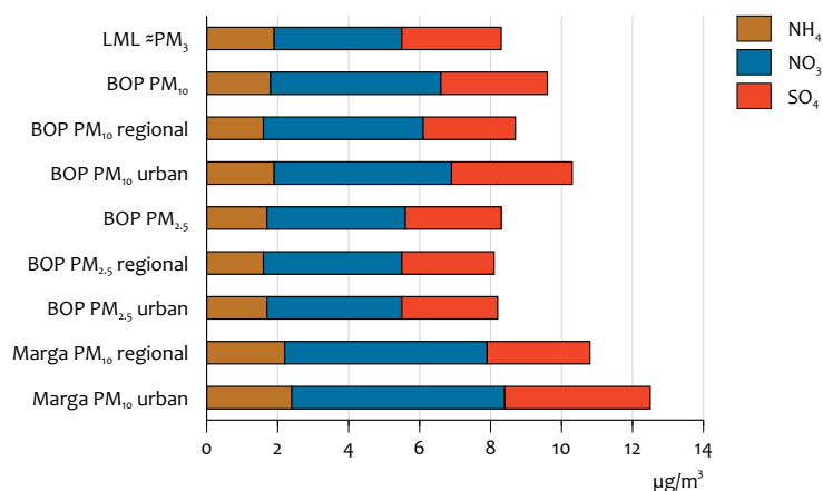
SIA overall, regional and urban averages for the LML, BOP and MARGA data sets
