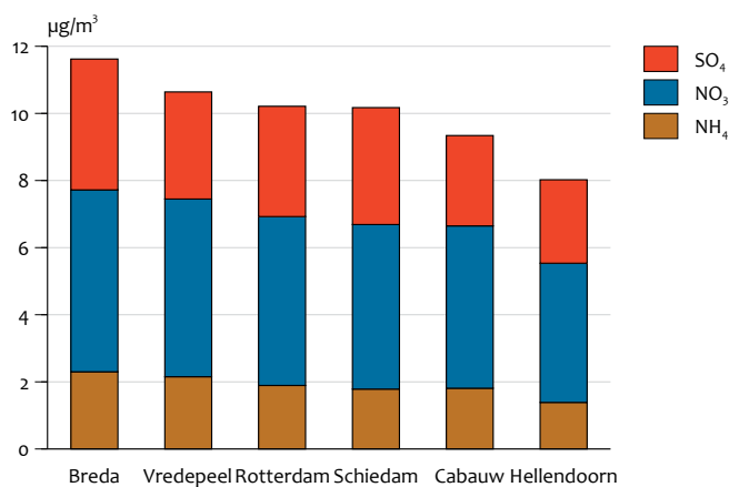
Average concentrations of NH 4 , NO 3 and SO 4 at six BOP locations
