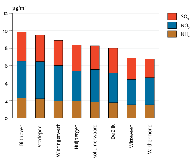
Average concentrations of \text{NH}_4 , \text{NO}_3 and \text{SO}_4 over 14 years at all LML sites
