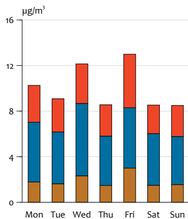
\text{PM}_{10} daily averages
