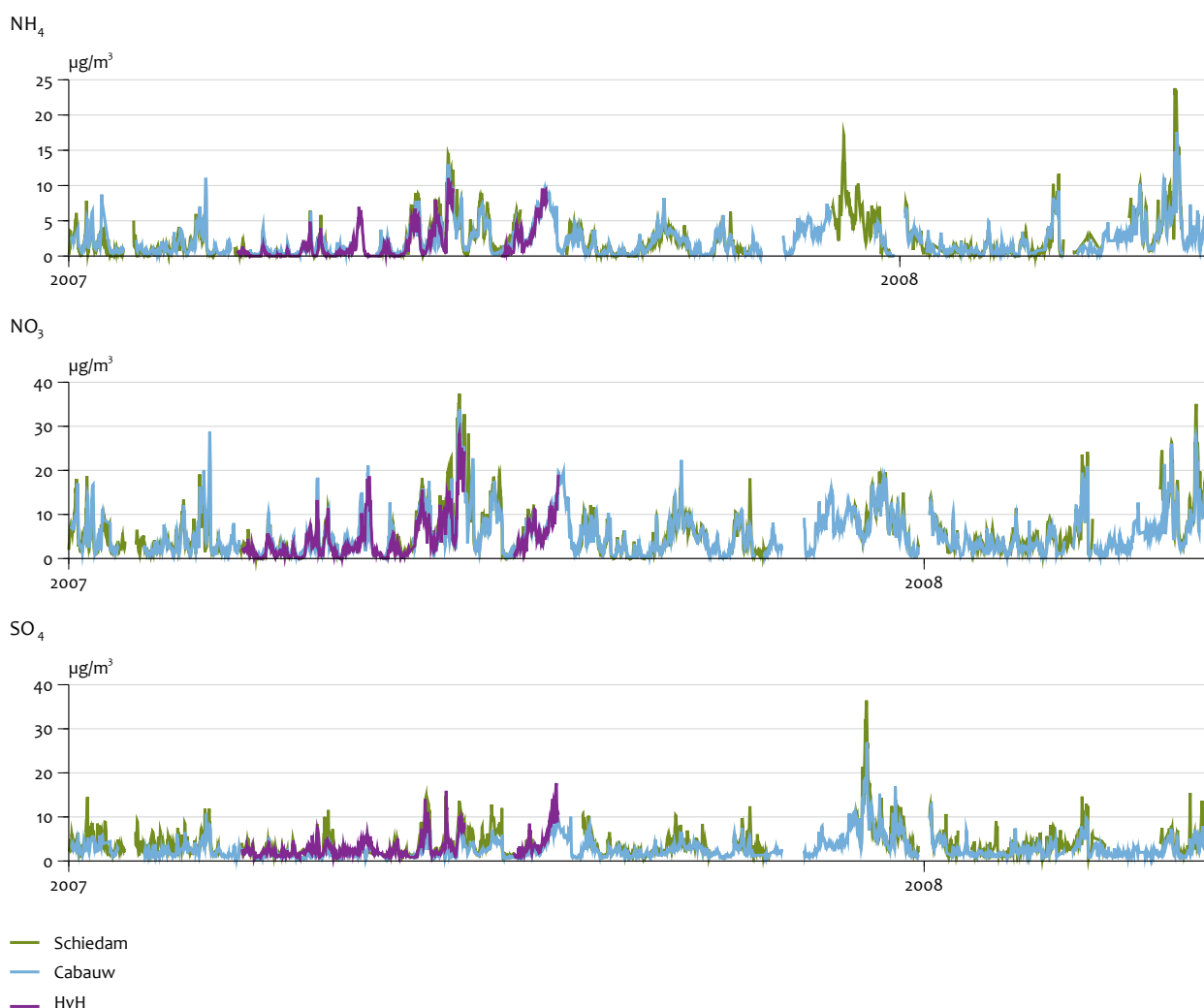
Time series of hourly NH 4 , NO 3 and SO 4 concentrations (MARGA) at the three locations
