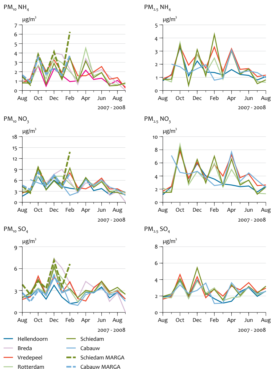
Monthly averages of \text{NH}_4 , \text{NO}_3 and \text{SO}_4 in \text{PM}_{10} and \text{PM}_{2.5} , over a one-year period, between 2007 and 2008, at all BOP sites.
