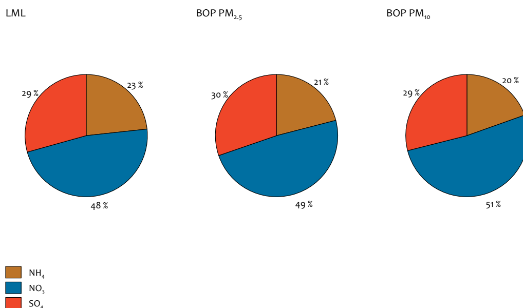
Percentual distributions of daily concentrations measured in LML network and BOP campaign at Vredepeel station Figure 5.3
