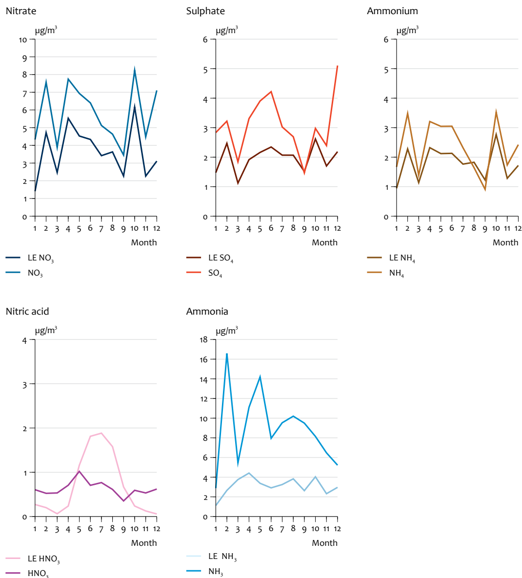
Modelled and measured seasonal cycle for nitrate, sulphate, ammonium, nitric acid and ammonia. Note that for easy interpretation the data have been organised as if it was a year from January to December. Hence, the monthly averages of January to July 2008, were put before the period of August to December 2007.
