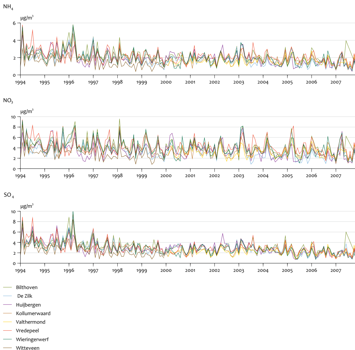
Time series of average monthly concentrations of LML data over 14 years.
