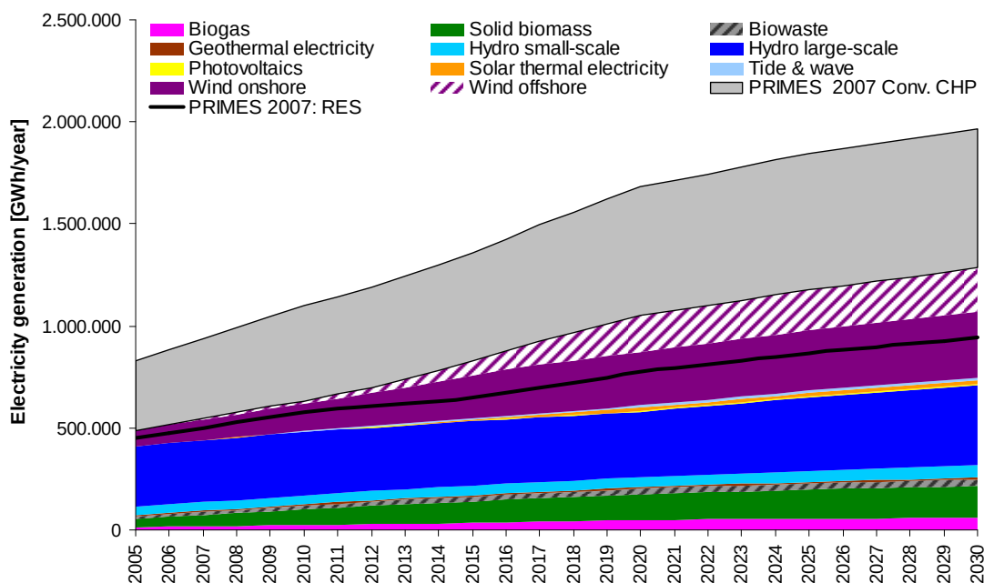
Figure 3.3: GreenNet BAU simulation results including projections until 2030 and conventional CHP updates for electricity generation on European level
