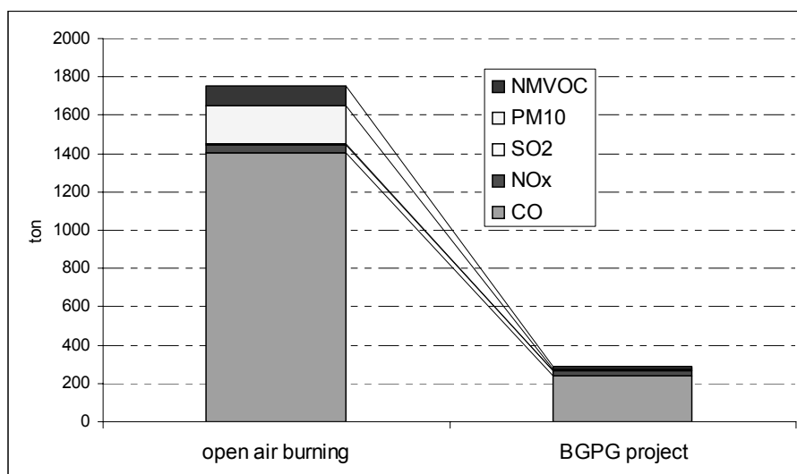
Figure 4-1: Emission of air pollutants related to open air burning of the same amount of biomass residue and from the BGPG project implementation
