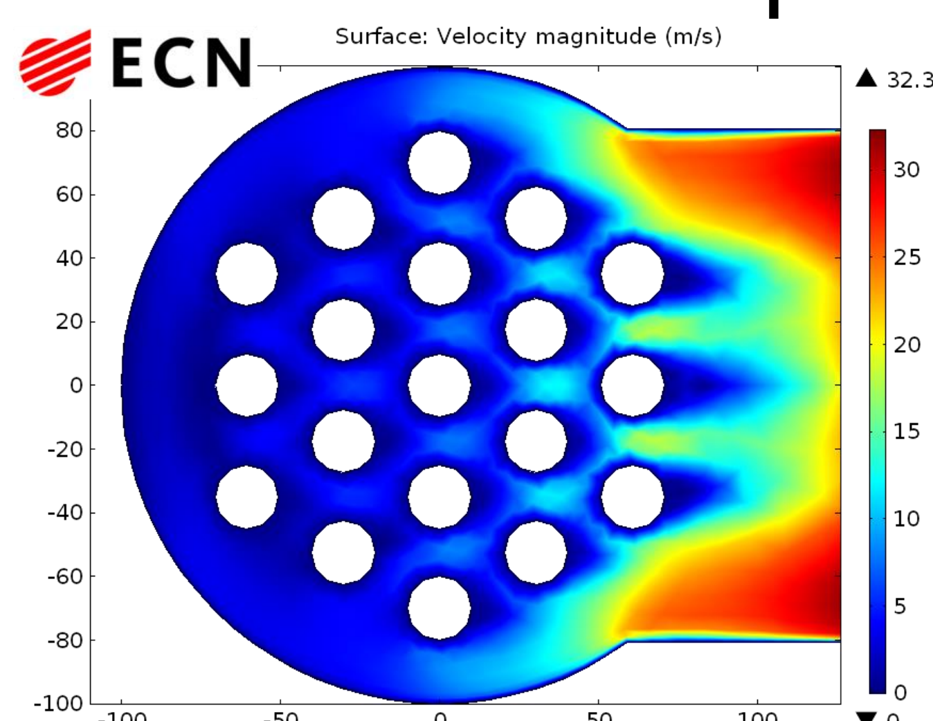
Figure 5. Velocity 19x4
