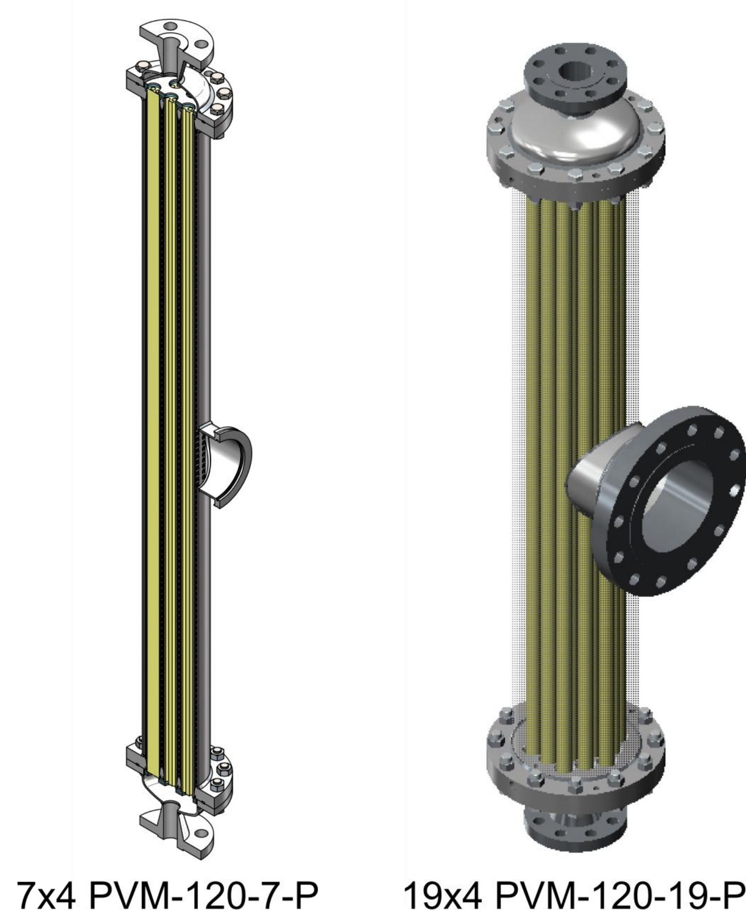
Figure 1. Pervaporation modules
