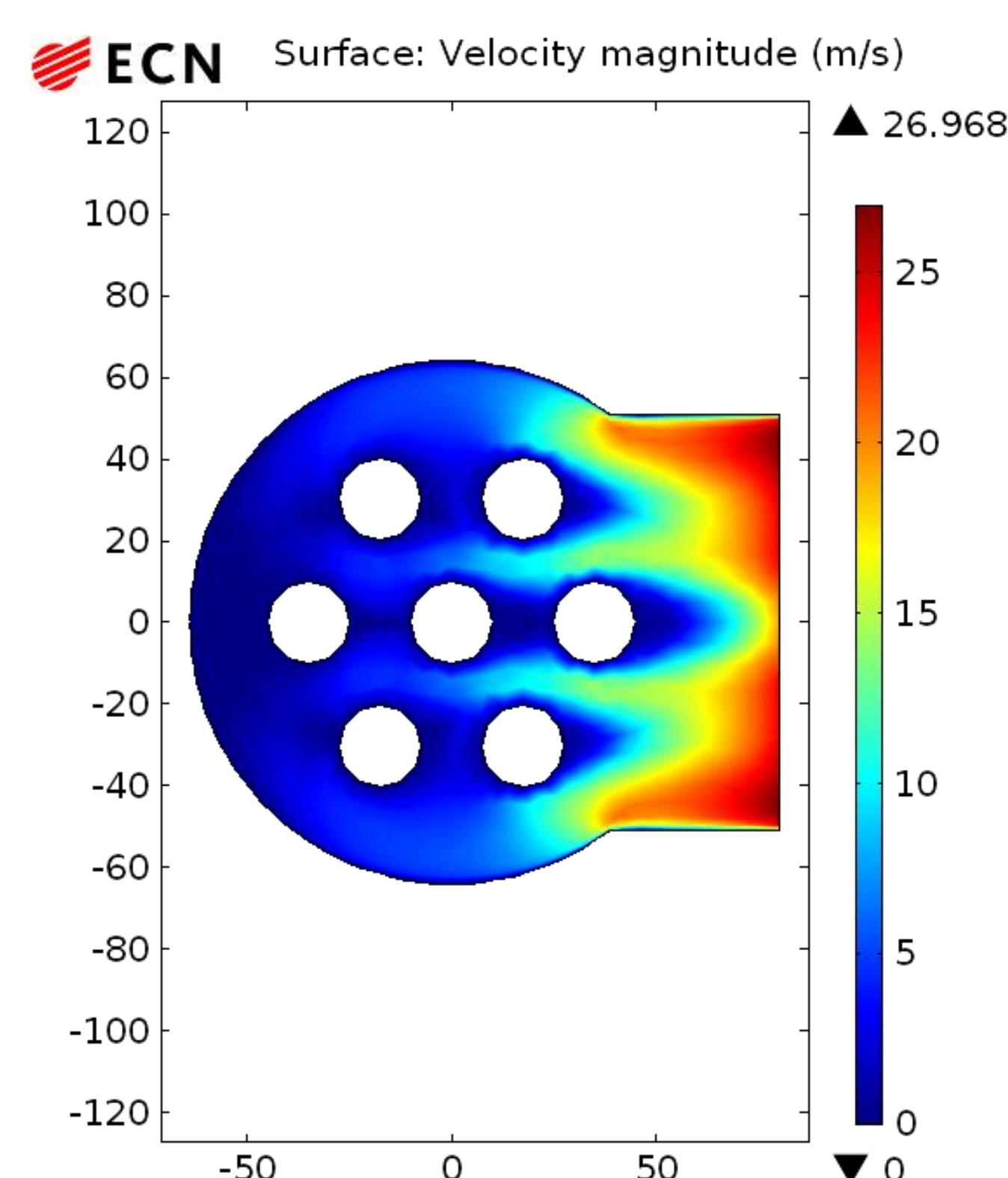
Figure 3. Velocity 7x4
