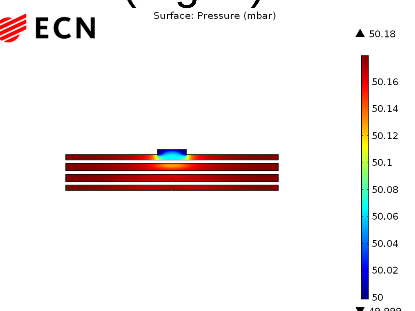
Figure 6. Pressure 19x4
