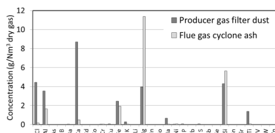
Figure 15: Composition of producer gas dust and flue gas cyclone ash generated in MILENA indirect gasification.
