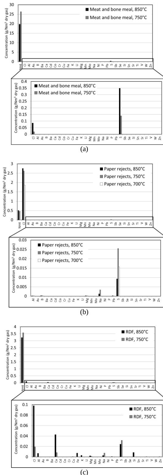
Figure 7: Effect of temperature on the gas phase composition of producer gas: (a) MBM gasification; (b) Paper rejects gasification; (c) RDF gasification.
