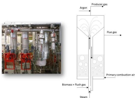
Figure 3: 25 \text{kW}_{\text{th}} MILENA gasifier at ECN.
