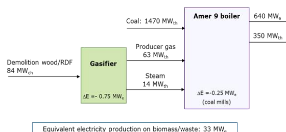
Figure 4: 80 \text{MW}_{\text{th}} CFB gasifier in Amercentrale 9 Essent plant, Geertruidenberg, Netherlands.
