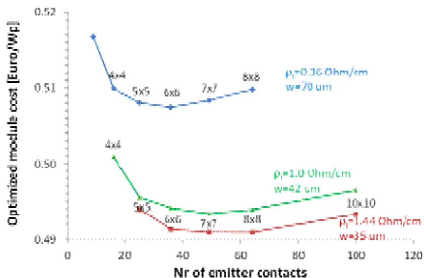
Figure 6: Optimised module cost for MWT cells with an increasing number of vias with different finger widths and line resistances. The reduced adhesive volume is included in these calculations. A cost reduction of close to 4% is predicted by going to a 6x6 or 7x7 via configuration in combination with a reduced finger width.
