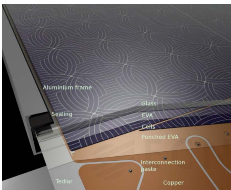
Figure 1: Cross-section through a back-contact module showing the patterned copper layer in the conductive back-sheet, the interconnection paste (i.e. conductive adhesive), the EVA perforated at the position of the interconnection paste and the MWT cells.
