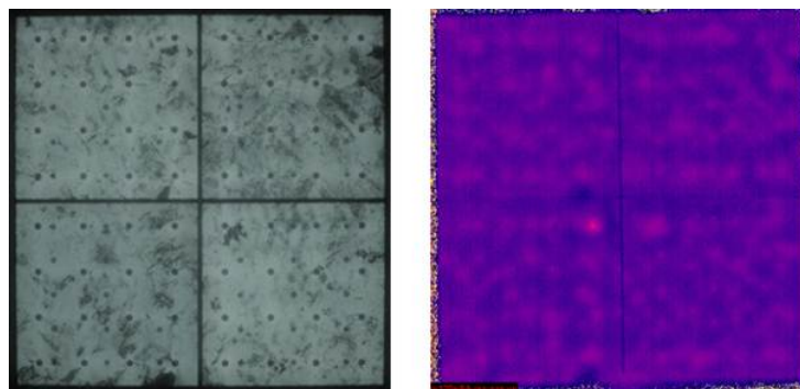
Figure 4: Left, EL image and, right, DLIT image of a four-cell module made with 100 µm thick encapsulant with a reduced volume of conductive adhesive. The images are uniform in colour and similar to images obtained from module made with 200 µm encapsulant and standard volume conductive adhesive contacts.
