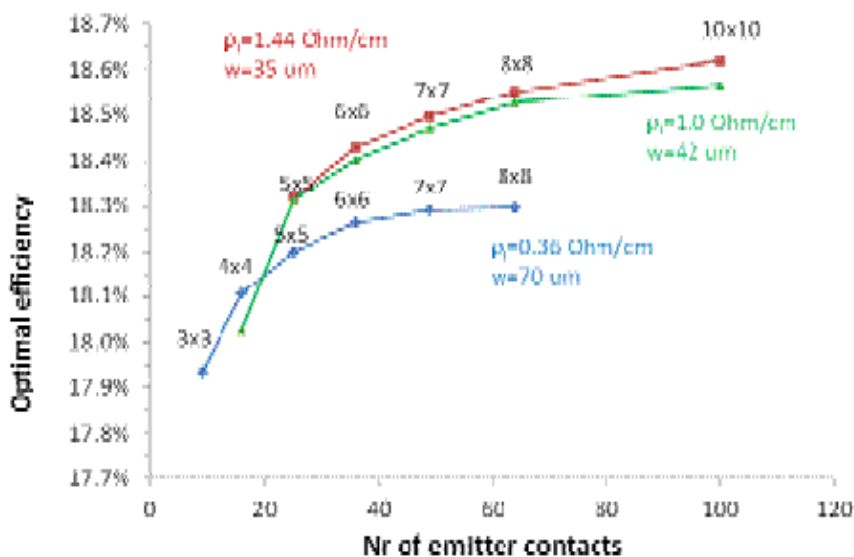
Figure 5: Modelling results for efficiency of MWT cells with an increasing number of vias with different finger widths and line resistances for the front side metallisation. The efficiency of the cell always increases with an increasing number of vias. Higher efficiencies can be achieved with narrower fingers for a higher number of vias.
