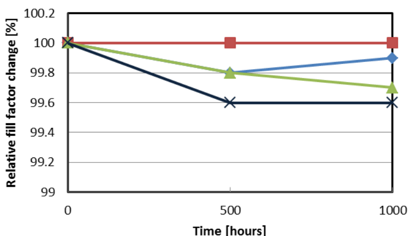
Figure 3: Damp-heat test results for mini-modules. The black line shows the reference module with a copper foil. The green line is a copper foil with copper cold-spray contacts. The red and blue lines are both aluminium with copper cold-spray conductive back-sheet foils. All foils show limited degradation up to 1000 hours in damp-heat (85%RH/85°C).
