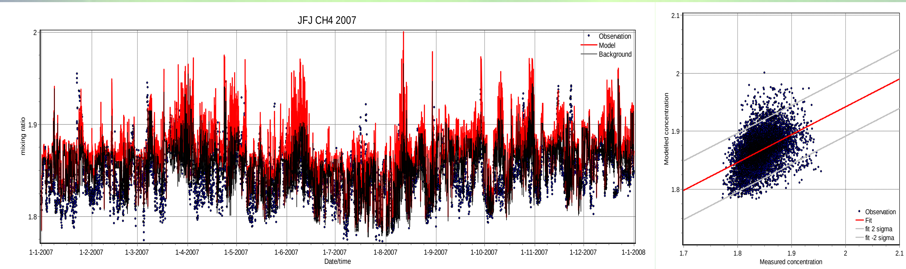
Fig 3 (a) Forward simulation and measured mixing ratios of CH 4 [ppm] at station Junkfraujoch in 2007 and (b) corresponding scatterplot of modeled versus measured mixing ratios [ppm]; see table 1
