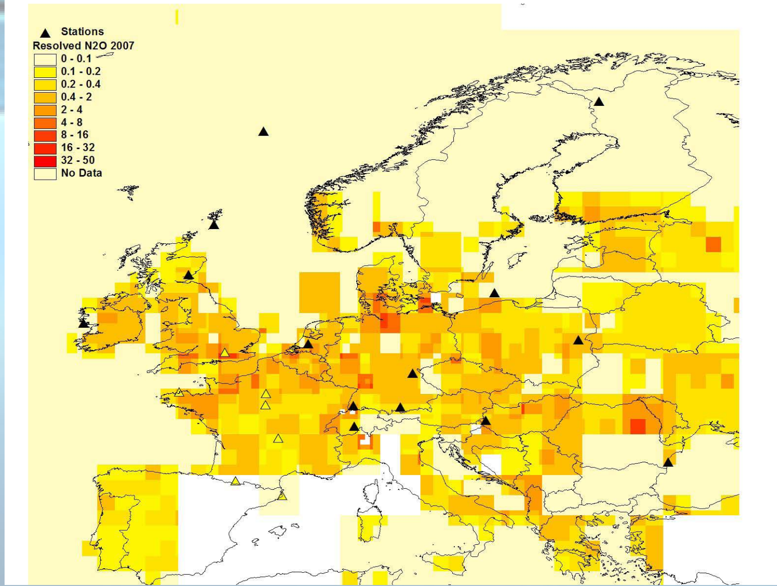
Fig 7 Posterior N 2 O emissions resolved from the observations in 2007 (at black triangles) using the COMET source area aggregation inversion system
