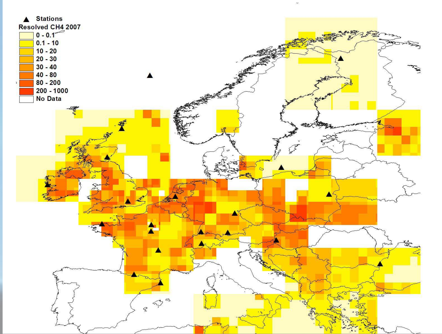
Fig 7 Posterior CH 4 emissions resolved from the observations in 2007 (at black triangles) using the COMET source area aggregation inversion system
