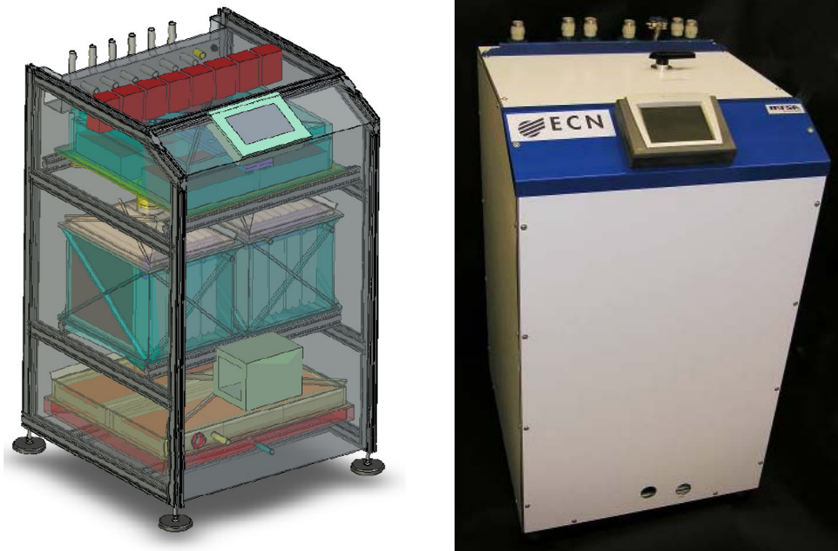
Figure 2: Design drawing and picture of the ECN 2.5 kW adsorption chiller
