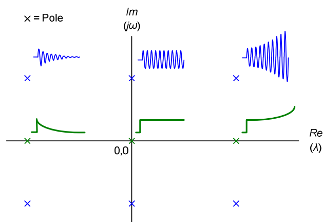
Figure 1, PZ-map and step-responses of a first- and second order system, resp. plotted in green and blue.
