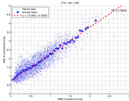
Figure 10: Correlation between turbulence measured at the nacelle of a N80 turbine and turbulence measured at a meteorological mast
