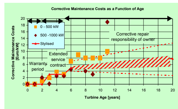
Figure 4: Development of the costs for unplanned corrective maintenance in the different stages of the lifetime [5].
