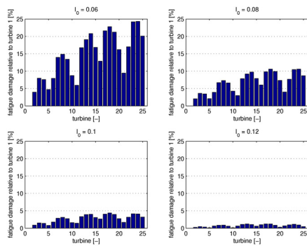
Figure 11: Relative fatigue damage (turbine 1 = reference) of the 25 turbines for different values of ambient turbulence intensity.
