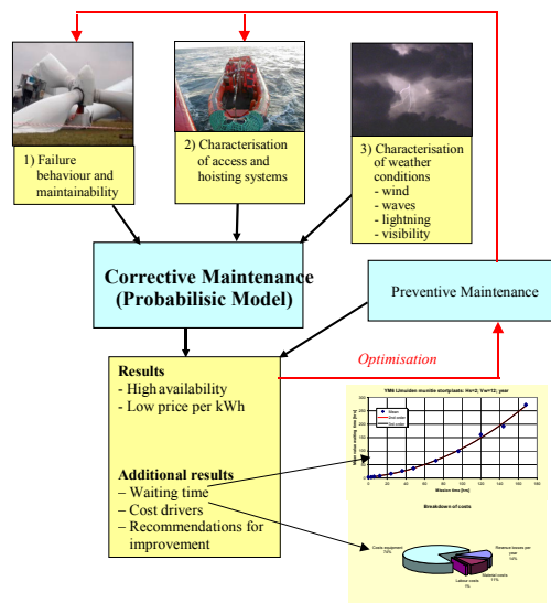
Figure 3: Schematic representation of the ECN O&M Tool for determining the O&M costs and downtime of an offshore wind farm.
