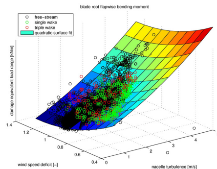
Figure 9: Correlation between turbulence, wind speed deficit and equivalent flapwise load ranges (using m = 7 ), measured at ECN wind turbine test site Wieringermeer
