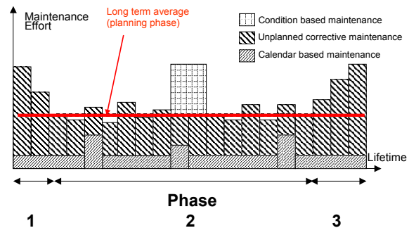
Figure 2: Schematic overview of the maintenance effort over the lifetime of an offshore wind farm.
