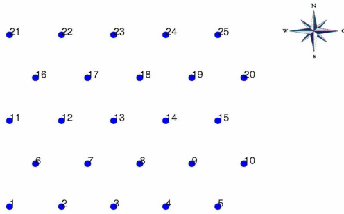
Figure 8: Layout of the fictitious 5x5 offshore wind farm of N80 turbines.
