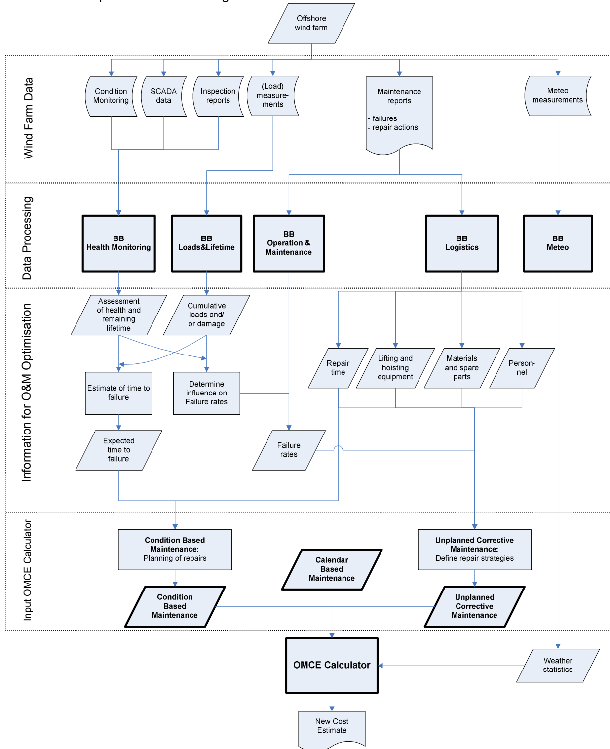
Figure 5: Structure for the O&M Cost Estimator.
