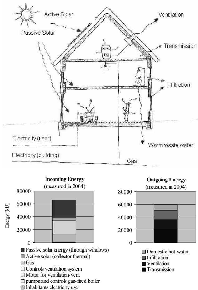
Figure 2: Incoming and outgoing energy flows (energy balance) measured in 2004 from a single-family dwelling with natural ventilation
