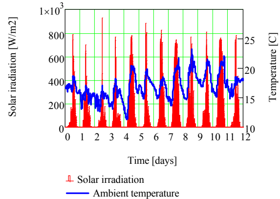
Figure 5: Solar irradiation on the south facade and ambient temperature during measurements with air cooling
