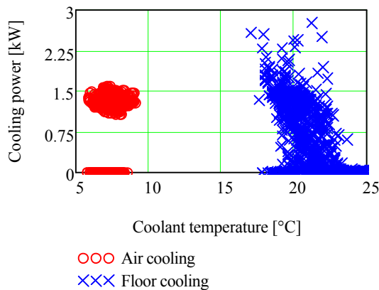
Figure 7: Cooling power and coolant temperature of both cooling systems during daytime in the living room
