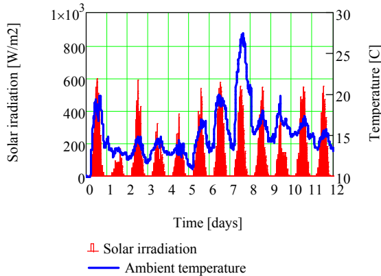
Figure 3: Solar irradiation on the south facade and ambient temperature during measurements with floor cooling
