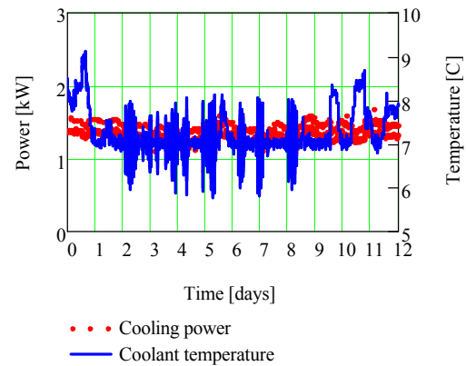
Figure 6: Cooling power and coolant temperatures during the measurements with air cooling
