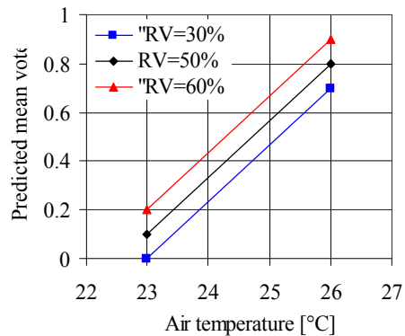
Figure 2: Influence of measured parameters on the PMV
