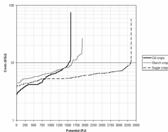
Figure 1: Cost-supply curves for first generation feedstock in 2010.
