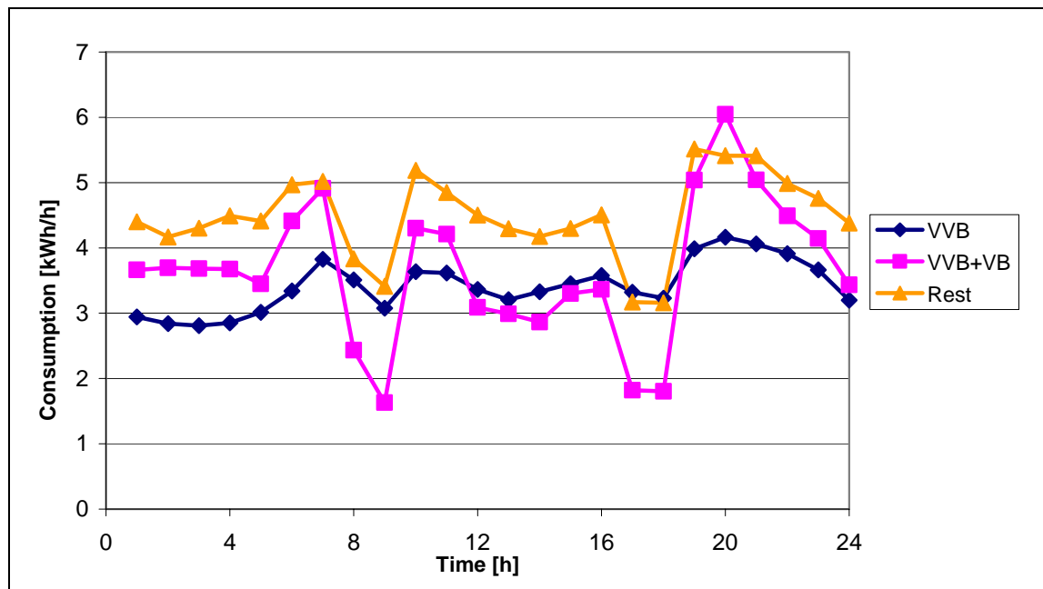
Figure 1 Load profiles for customers with remote load reduction. Source: SINTEF Energiforskning AS, project MabFot
