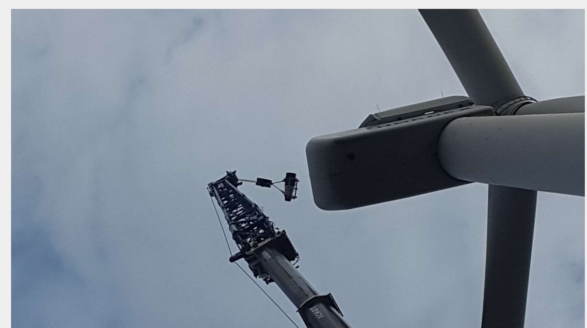
Hoisting the the SpinnerLidar to the Nordex wind turbine at ECN
