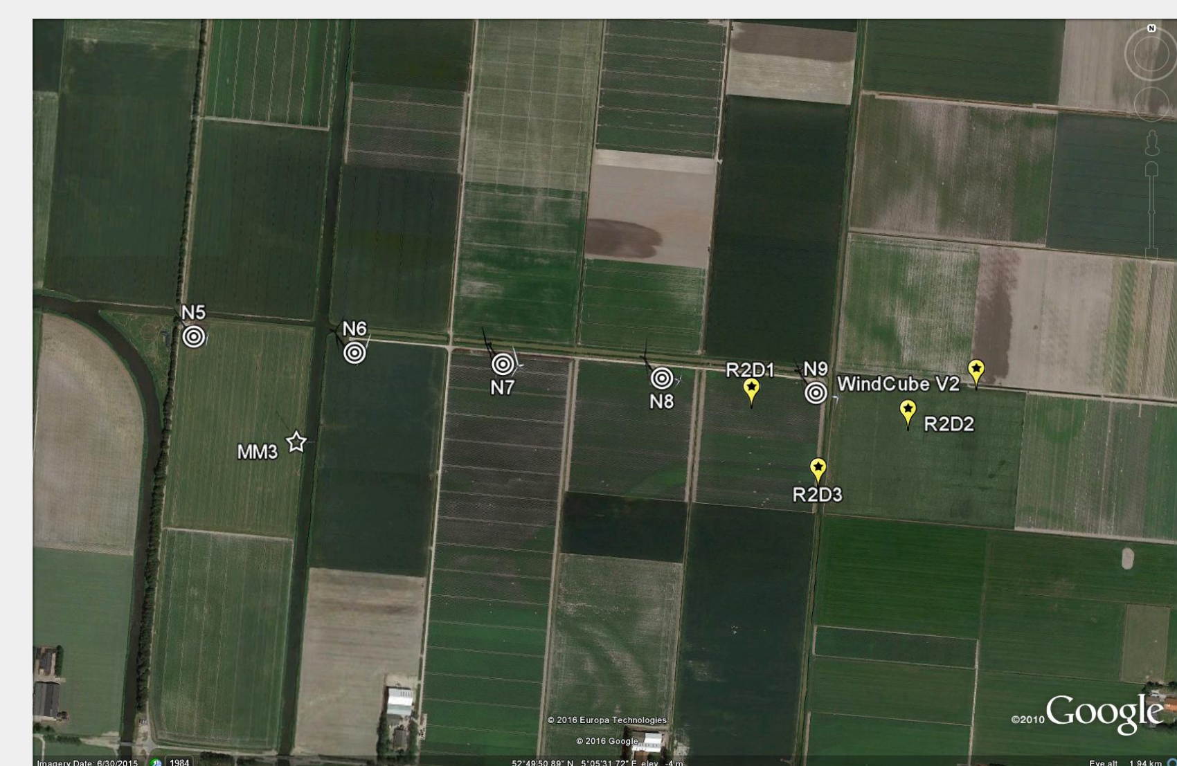
ECN Test Site with 5 research turbines in flat agricultural terrain.
