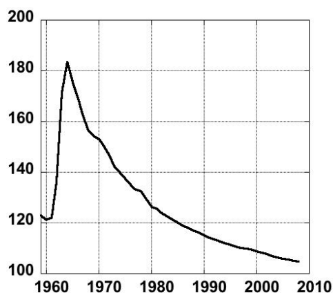
Figure 3. — Decrease in ^{14}\text{C} value atmospheric air \text{CO}_2 (in pMC), measured at High Alpine Stations Vermunt (Austria) and Jungfrauoch (Switzerland). Data has been published in [8]
