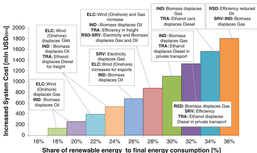
Fig. 3 Illustrative cost supply curve for Ireland. Information on the x-axis and y-axis show the share of RE in TFFC and the increased system costs, respectively
