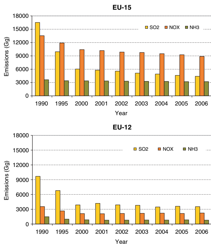
Figure 4.5. Changes in total \text{NO}_x and \text{NH}_3 emissions to air in EU-15 (top) and EU-12 (bottom) between 1990 and 2006. Emissions of \text{SO}_2 to air are shown for comparison (source: EEA, 2008).
