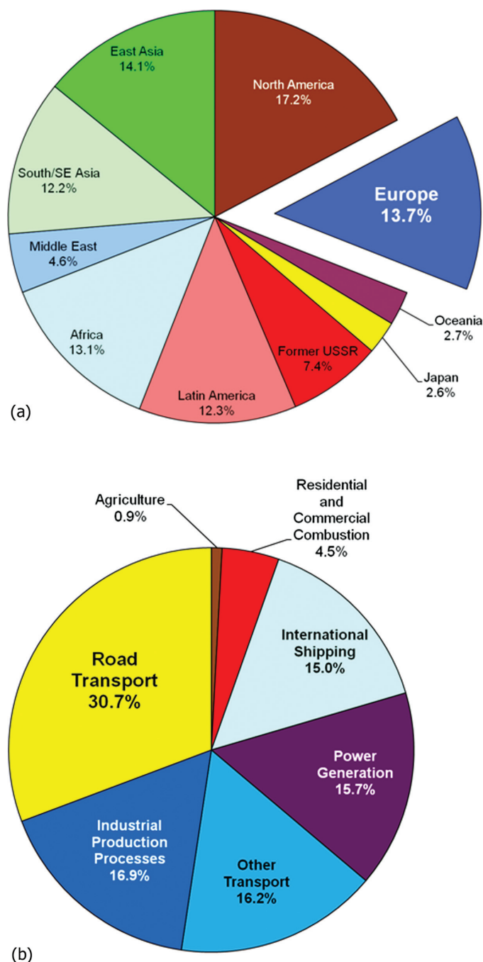
Figure 2.9 NO x contribution by different regions of the world (a) and different sources (b), based on EDGAR data for the year 2000 (EDGAR, 2010).
