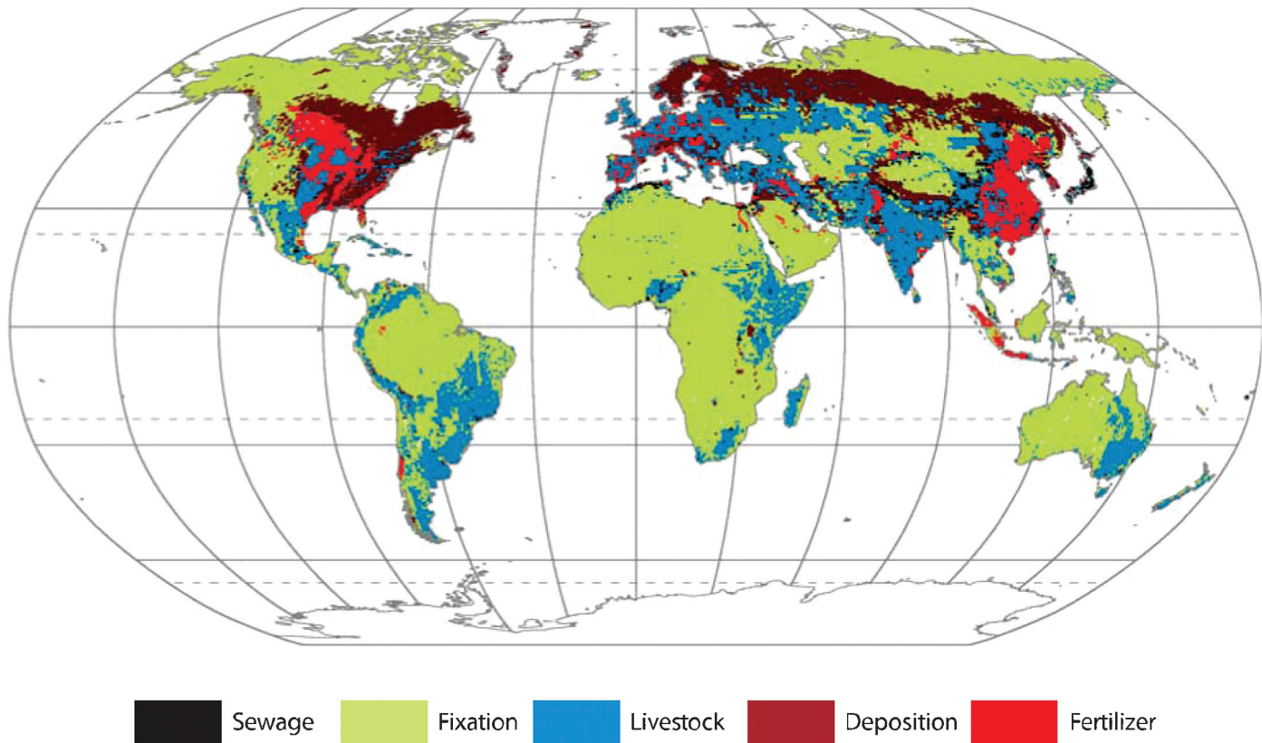
Figure 2.13 Nitrogen loading onto the land mass and aquatic systems as a source for delivery to the coastal zone; a measure of potential water pollution. Total and inorganic nitrogen loads as deposition, fixation, fertilizer, livestock loads, human loads and total distributed nitrogen to the land and aquatic system. Map prepared by Water Systems Analysis Group, University of New Hampshire.
