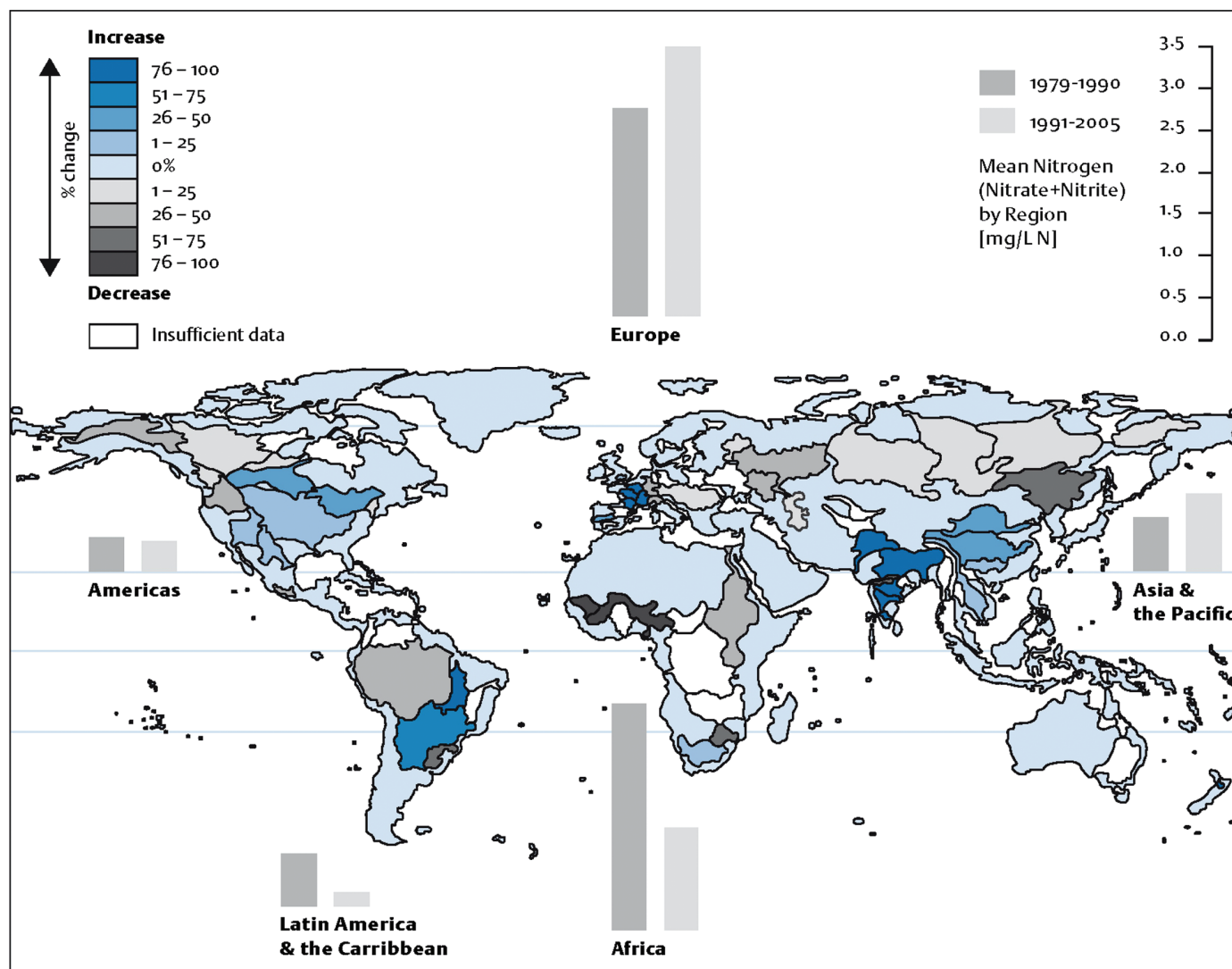
Figure 2.15 Changes in nitrogen concentrations for significant global watersheds (percentage) and by region (concentration): 1979–1990 and 1991–2005 (UNEP GEMS, 2006).
