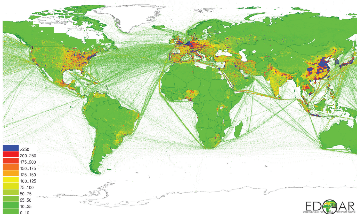
Figure 2.8 Global emissions of nitrogen oxides ( \text{NO}_x ) (EDGAR, 2010).
