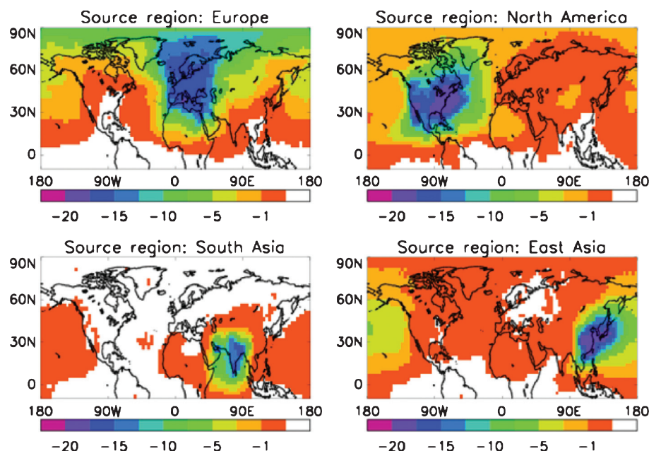
Figure 2.10 The transport distance of \text{NO}_x emissions of Europe and North America over the globe. Shown is the percentage change in deposition of \text{NO}_y in each \text{NO}_x emission perturbation experiment relative to the control run, using multi-model annual mean deposition fluxes (Sanderson et al. , 2008).
