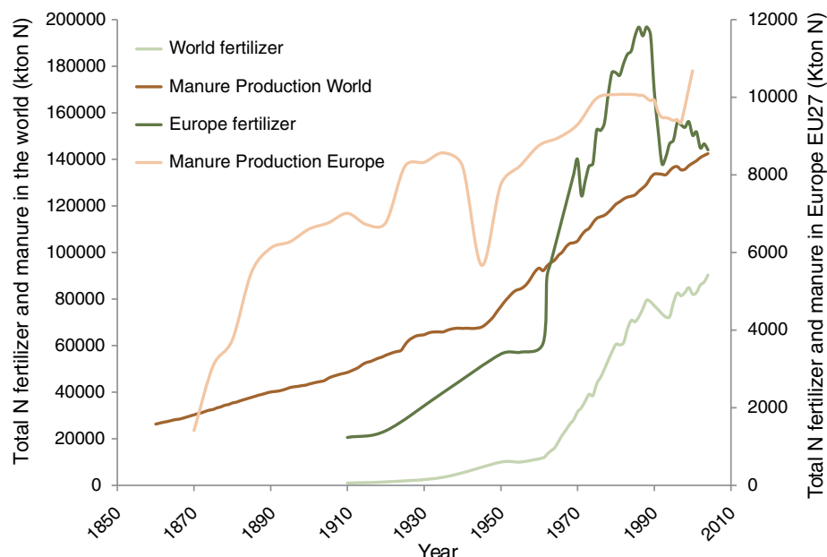
Figure 2.4 Global and European livestock manure and fertilizer nitrogen consumption (Kton N). Global data are obtained from Davidson (2009). European data are constructed from animal numbers and excretion factors by Buijsman (1986) and the INTEGRATOR model (de Vries et al. , 2009).
