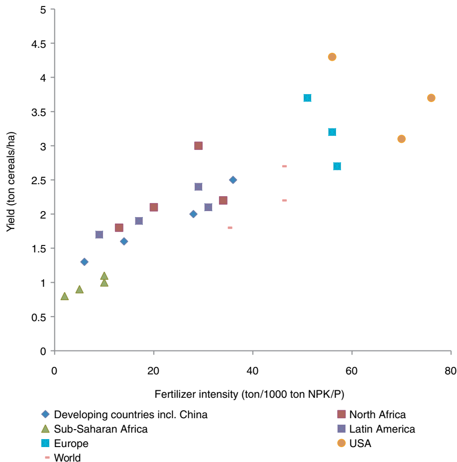
Figure 2.3 Overall yield (Y) and fertilizer intensities (FI) for the developing regions, and other countries and regions between 1960 and 1990. The fertilizer intensity is the fertilizer input (expressed as the amount of N + P 2 O 5 + K 2 O) as a fraction of total biomass production (FAO, 2010a).
