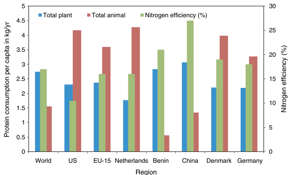
Figure 2.7 Protein consumption per capita as direct nitrogen intake in kg/yr in 1995 for different regions of the world and the nitrogen efficiency of protein consumption relative to N inputs (%) (van Grinsven et al. , 2003).
