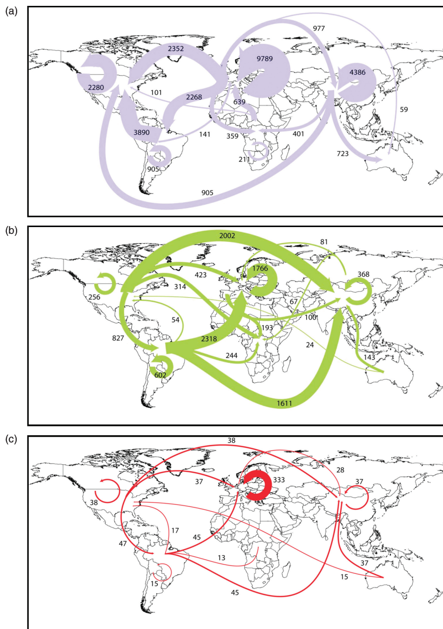
Figure 2.12 Amounts of N contained in internationally traded products: (A) fertilizer (31 Tg N), (B) grain (12 Tg N), and (C) meat (0.8 Tg N). Data are for 2004 and are in units of thousand of tons. Minimum requirements for drawing a line are 50 000 tons N, 20 000 tons N and 10 000 tons N for fertilizer, grain and meat respectively (UNEP, 2007; Galloway et al. , 2008).
