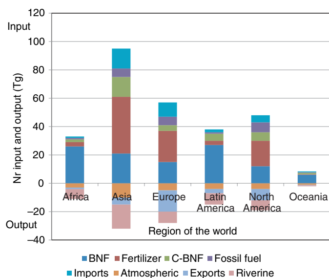
Figure 2.11 Nitrogen input and output (Tg) for different regions of the world (data from Galloway et al. , 2004).
