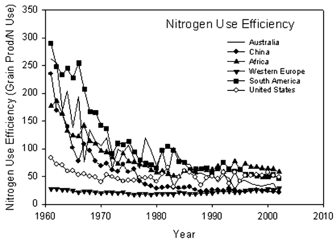
Figure 2.6 Nitrogen use efficiency for grain production relative to N fertilizer use for 1961–2002 for selected regions in the world (Hatfield and Prueger, 2004). Data source is http://faostat.fao.org/faostat .
