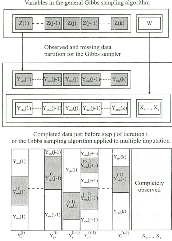
Figure 4-3: The Gibbs sampling algorithm for generating imputations.
