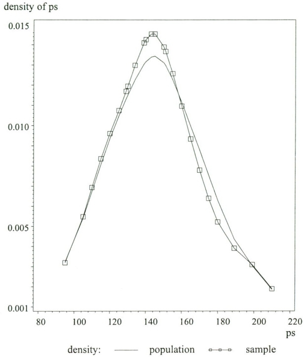
Figure 4-4: Kernel estimates of population and sample.
