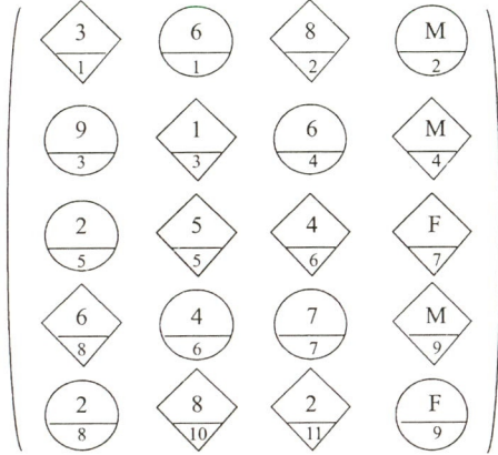
Figure 2-4: One possible definition of y_{\text{obs}} , y_{\text{mis}} and R .
