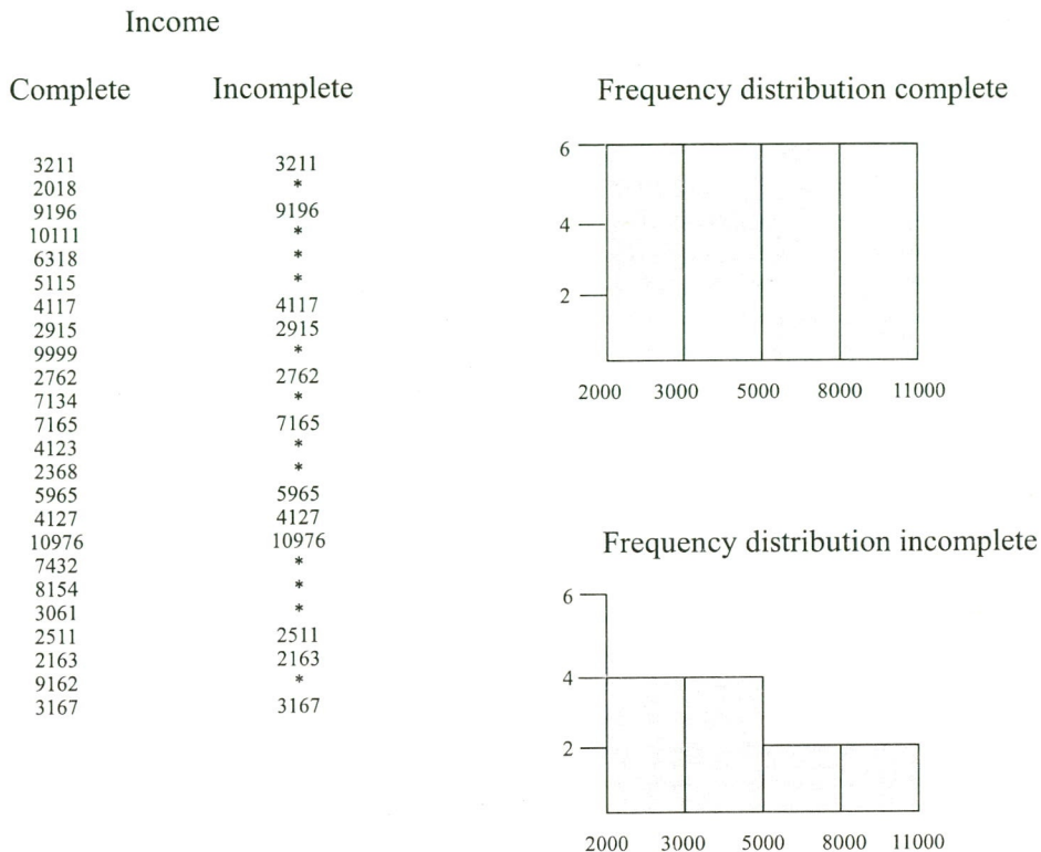
Figure 2-2: An example of an MNAR missing data mechanism.
