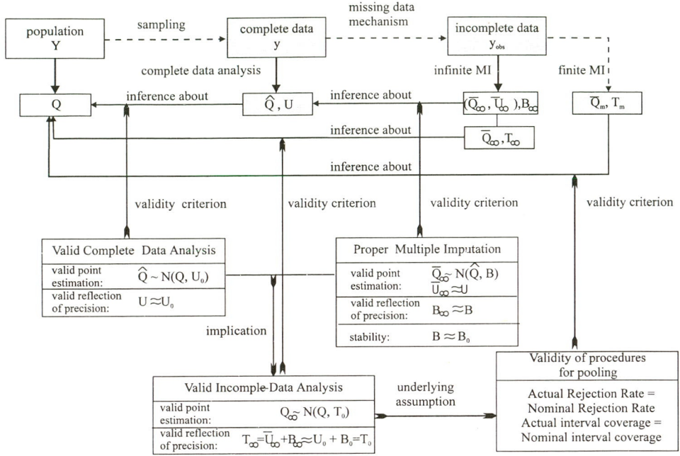
Figure 4-9: An overview of the validity criteria for complete data inference, incomplete data inference and multiple imputation.
