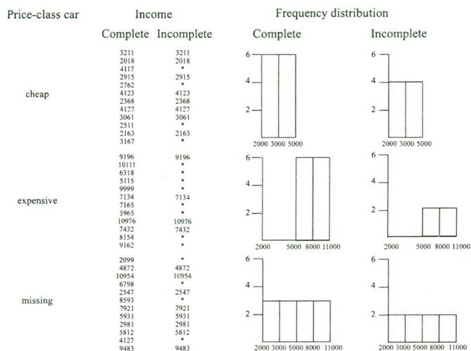
Figure 2-8: An example of a MAR missing data mechanism in which the probability of a missing data entry depends on incomplete covariates.
