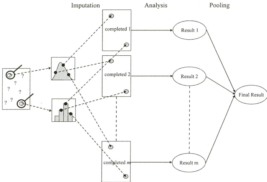
Figure 4-2: The concept of multiple imputation.
