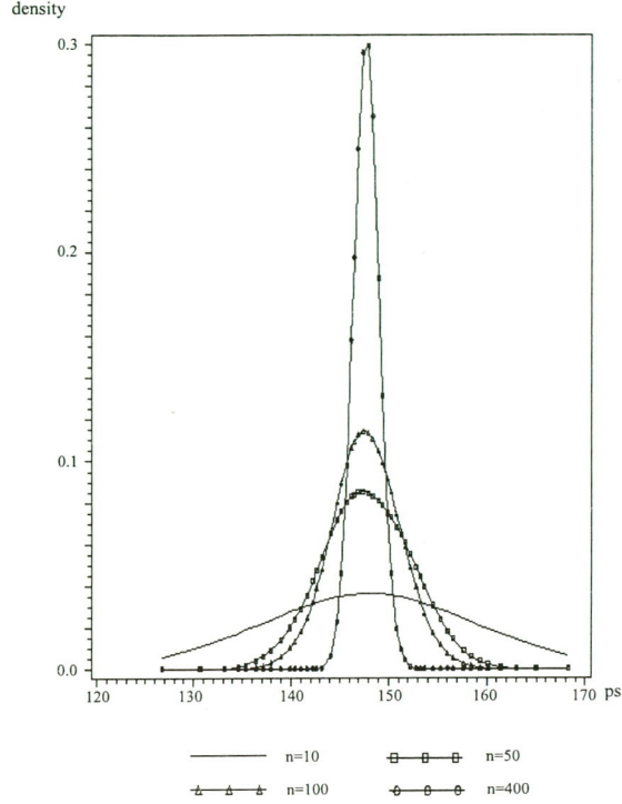
Figure 4-5: Distributions of sample means for different sample sizes.
