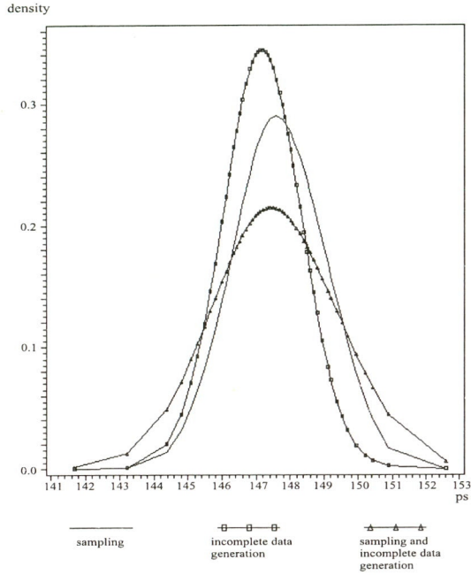
Figure 4-7: Kernel estimates of probability density distributions of \hat{Q} under repetition of sampling, \bar{Q}_\infty under repetition of generating incomplete data sets from a fixed complete data set, and \bar{Q}_\infty under repetition of sampling and generation of incomplete data sets, represented by solid graphs, graphs with squares, and with triangles, respectively.
