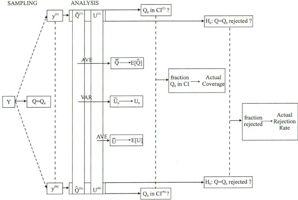
Figure 4-6: Setup for a Monte Carlo evaluation of complete data inference. The terms AVE and VAR represent the sample average and variance, respectively.
