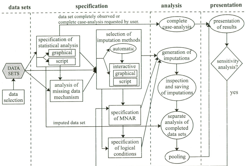
Figure 6-2: A conceptual model for a missing data engine. Rectangular objects represent steps that are executed interactively, and oval objects those that are executed without interaction. Steps that have been realized so far and those that remain to be implemented in future are represented by shaded and unshaded objects, respectively. The collection of available data sets is represented by the dark-shaded hexagon.
