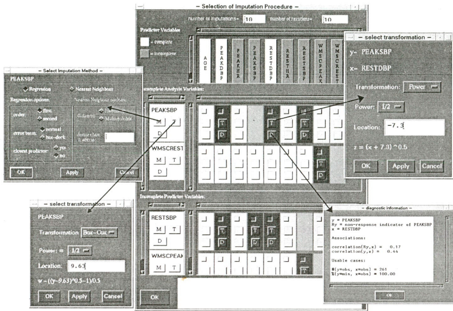
Figure 6-7: The graphical user interface for the interactive specification of an imputation method.
