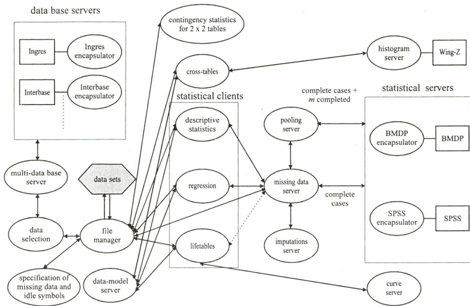
Figure 6-6: Architecture of the missing data engine in HERMES.
