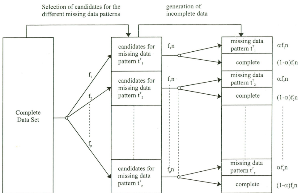
Figure 5-1: Schematic overview of the generation of incomplete data sets.
