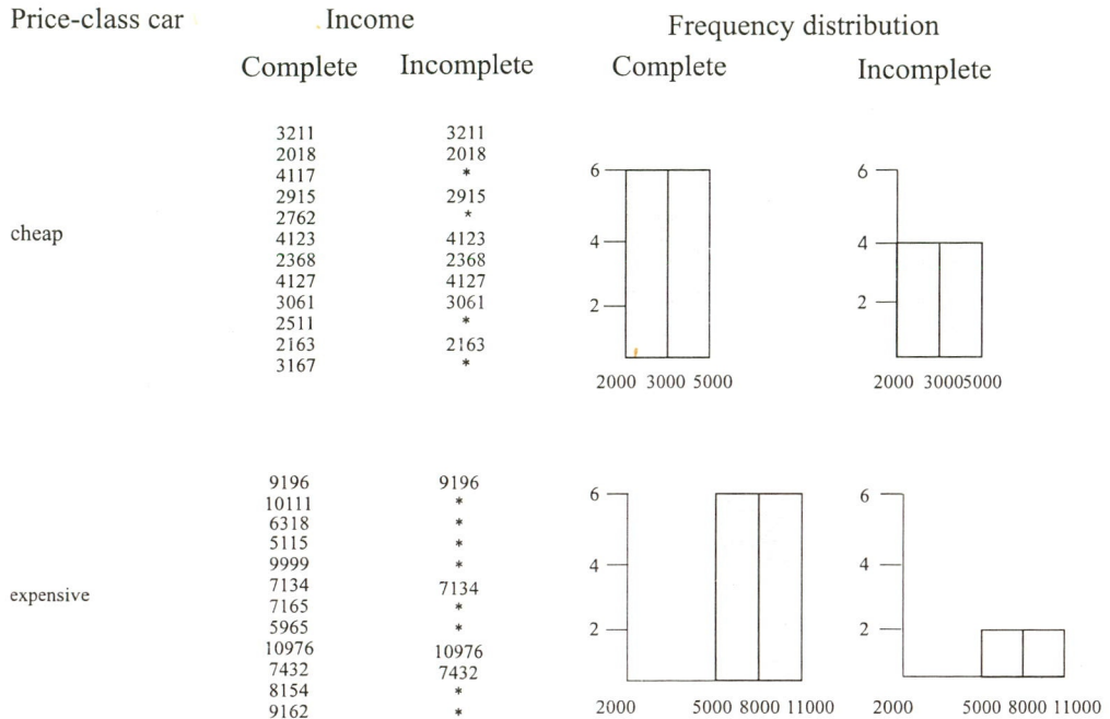
Figure 2-3: An example of a MAR missing data mechanism.
