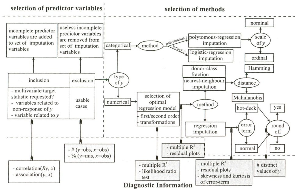
Figure 6-1: Schematic overview of the interactive selection of a multiple imputation procedure.
