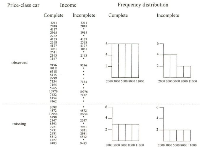
Figure 2-9: Frequency distributions for the complete and incomplete incomes of the employees with observed and missing values for the class of the car.
