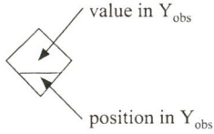
Figure 2-4: One possible definition of y_{\text{obs}} , y_{\text{mis}} and R .
