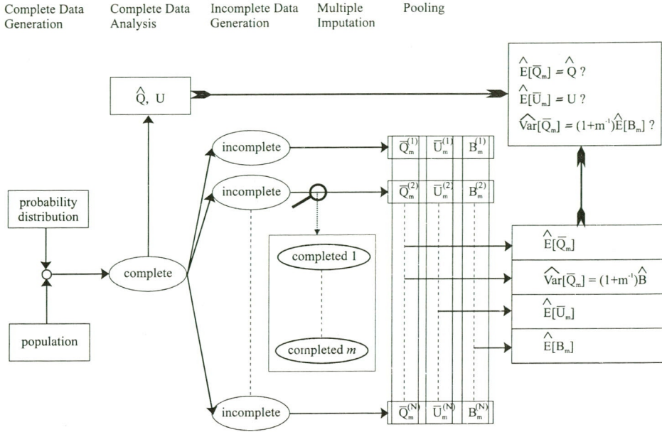
Figure 5-2: A schematic overview of the verification of proper multiple imputation.
