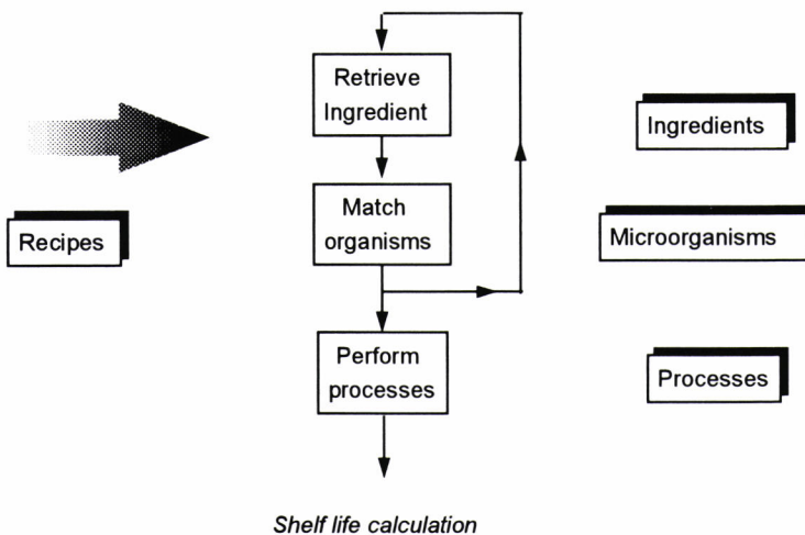
FIG. 3. Food design support system (FDSS), program flow.
