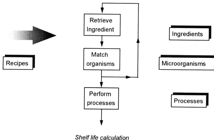
FIG. 5. Inference scheme FDSS.
