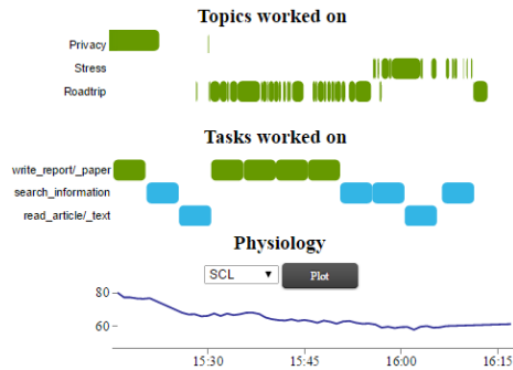
Figure 1: SWELL-KW dataset browser (extract). Topic and task worked on depicted (green: main task, blue: help task), together with the skin conductance level (measure of stress).
